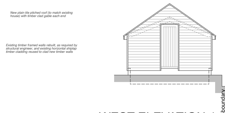
WEST ELEVATION 1:100
