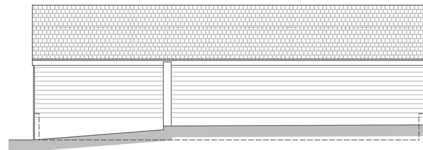
NORTH ELEVATION 1:100
