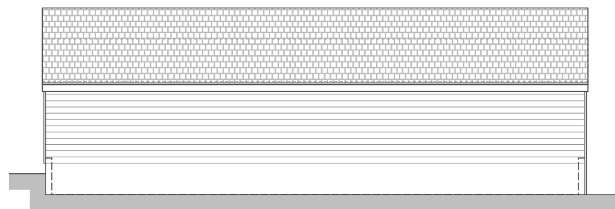
SOUTH ELEVATION 1:100
