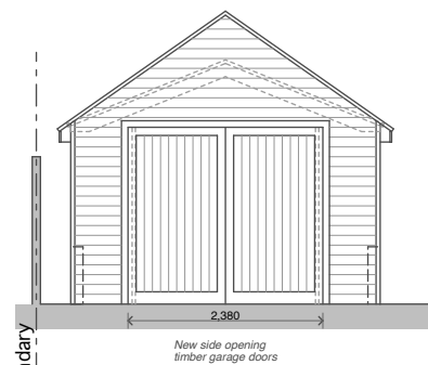
EAST ELEVATION 1:100
