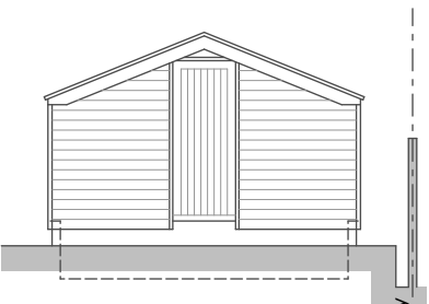
WEST ELEVATION 1:100
