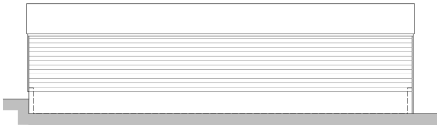
SOUTH ELEVATION 1:100
