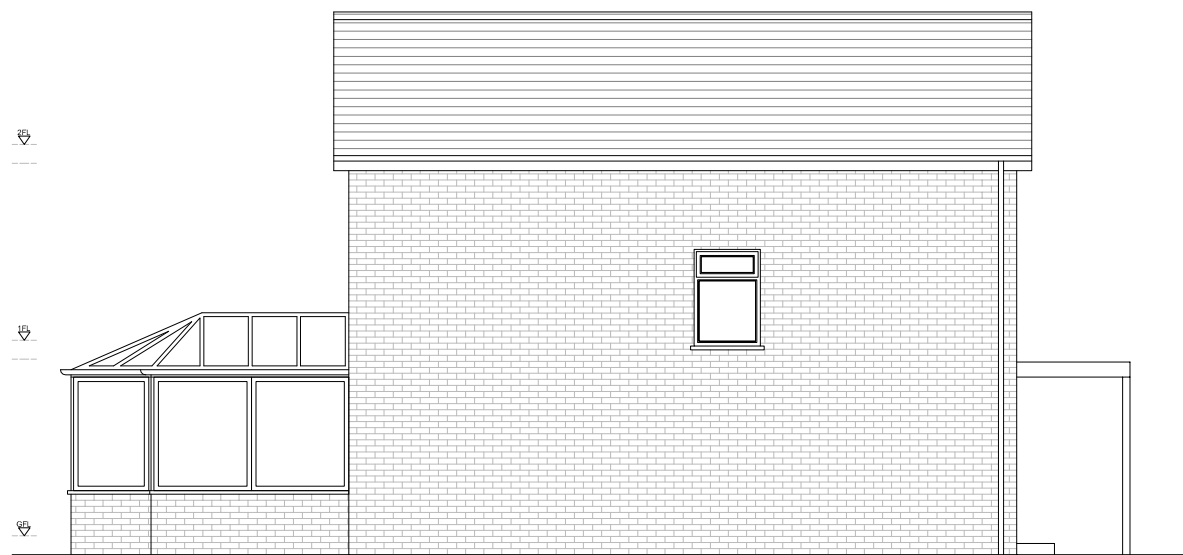
EXISTING SIDE (WEST) ELEVATION scale 1:100
