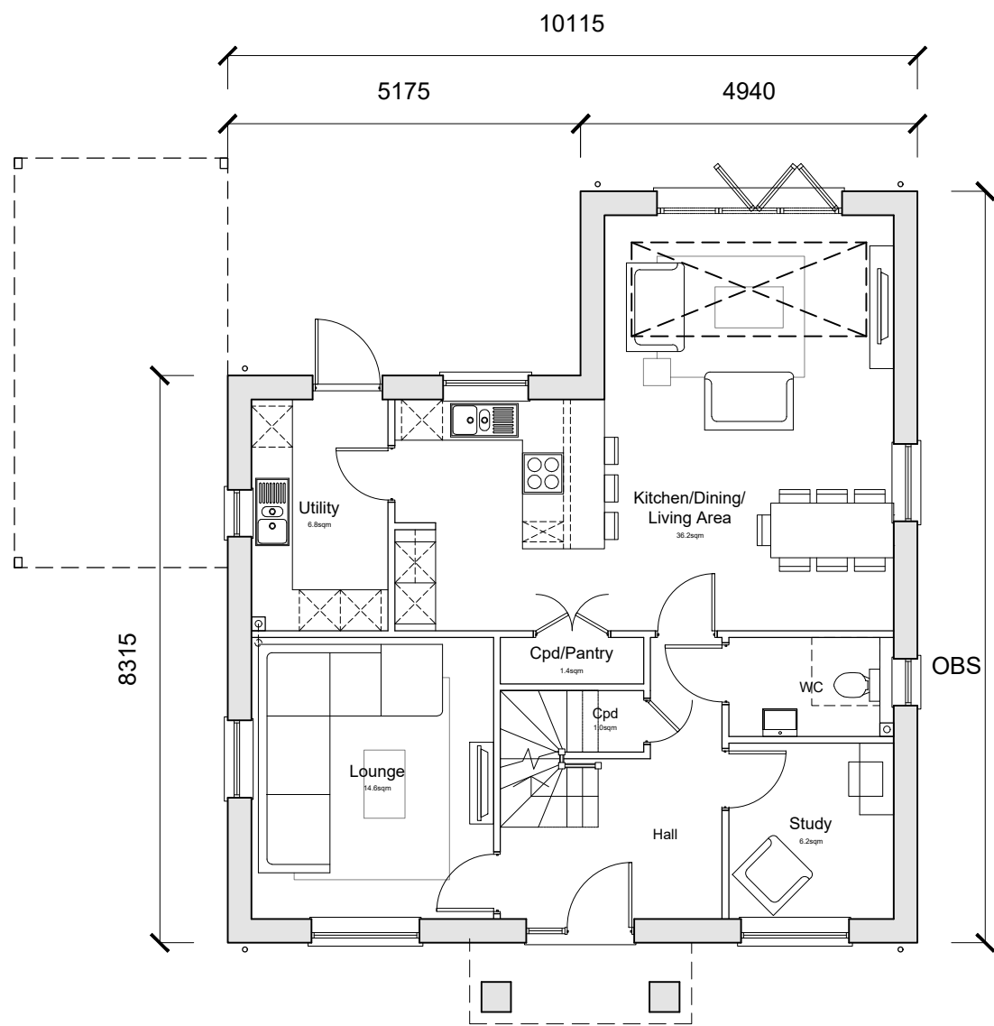
Ground Floor
