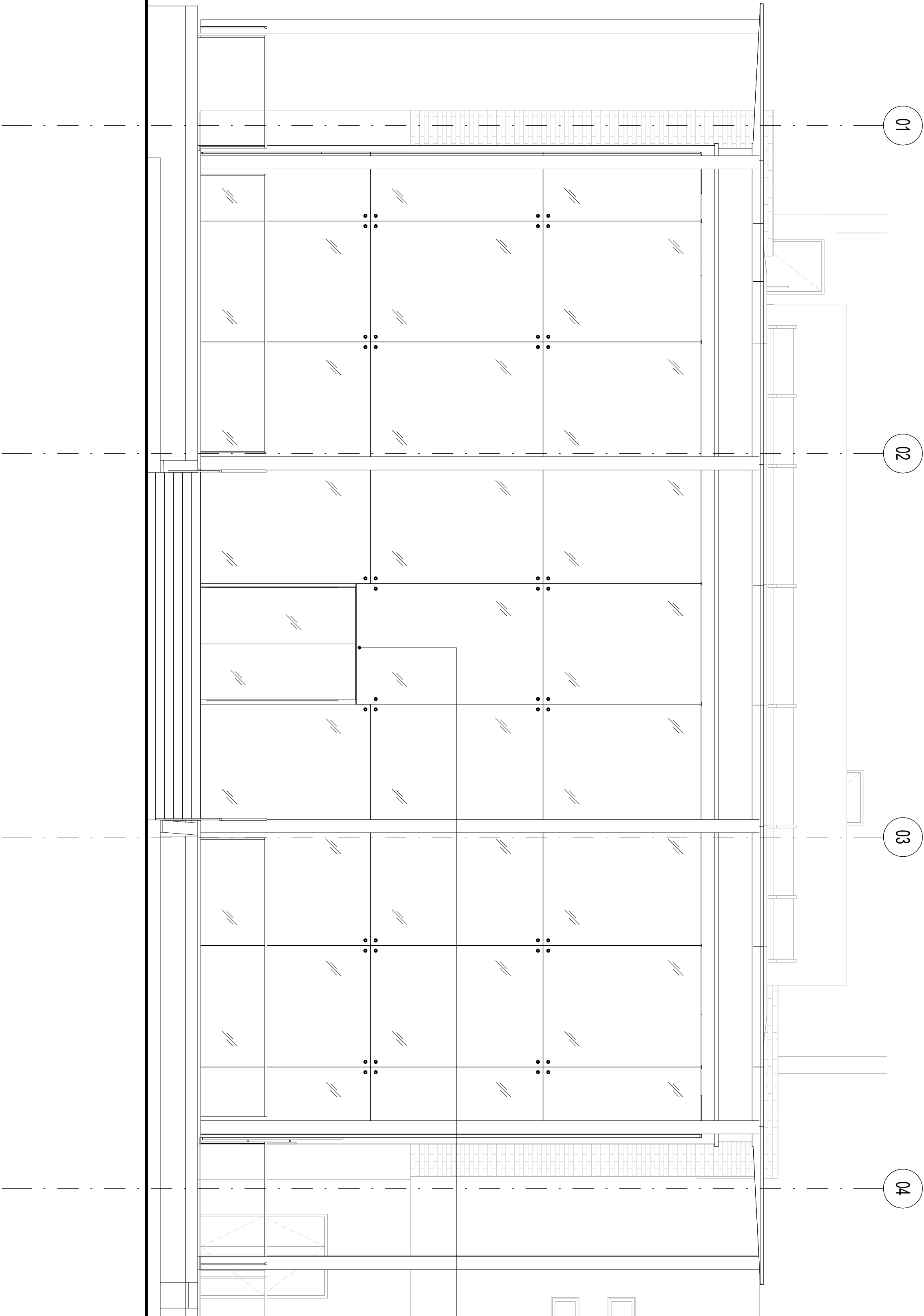
1 Existing - Glass Revolving Door 1 : 50
