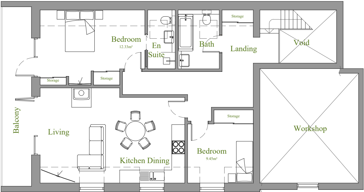
First Floor Plan 1:100 | APPROVED
