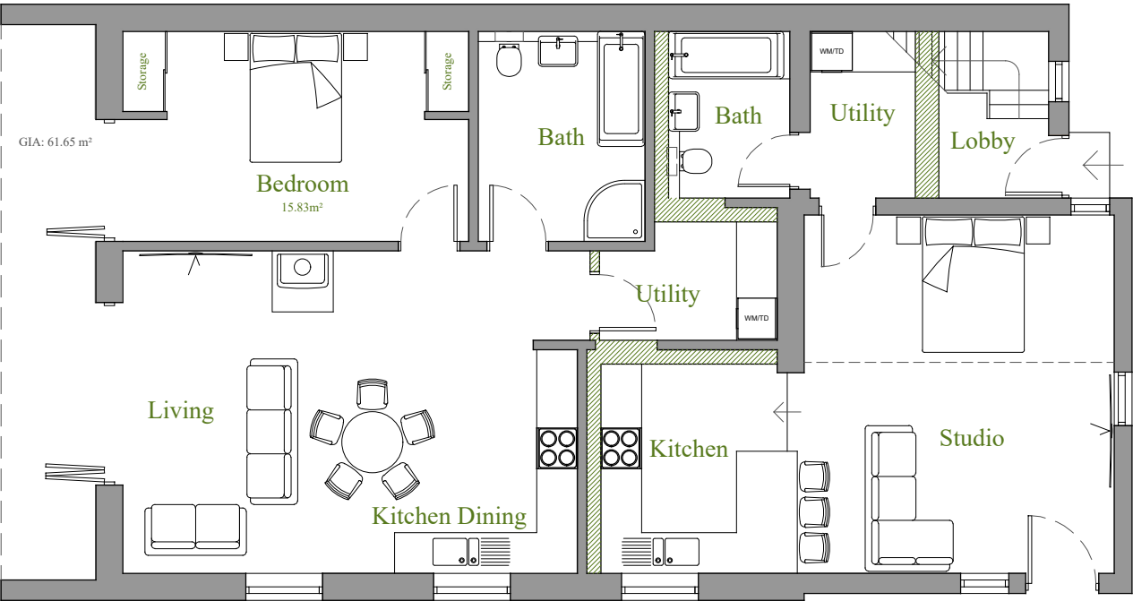
Ground Floor Plan 1:100 | PROPOSED
