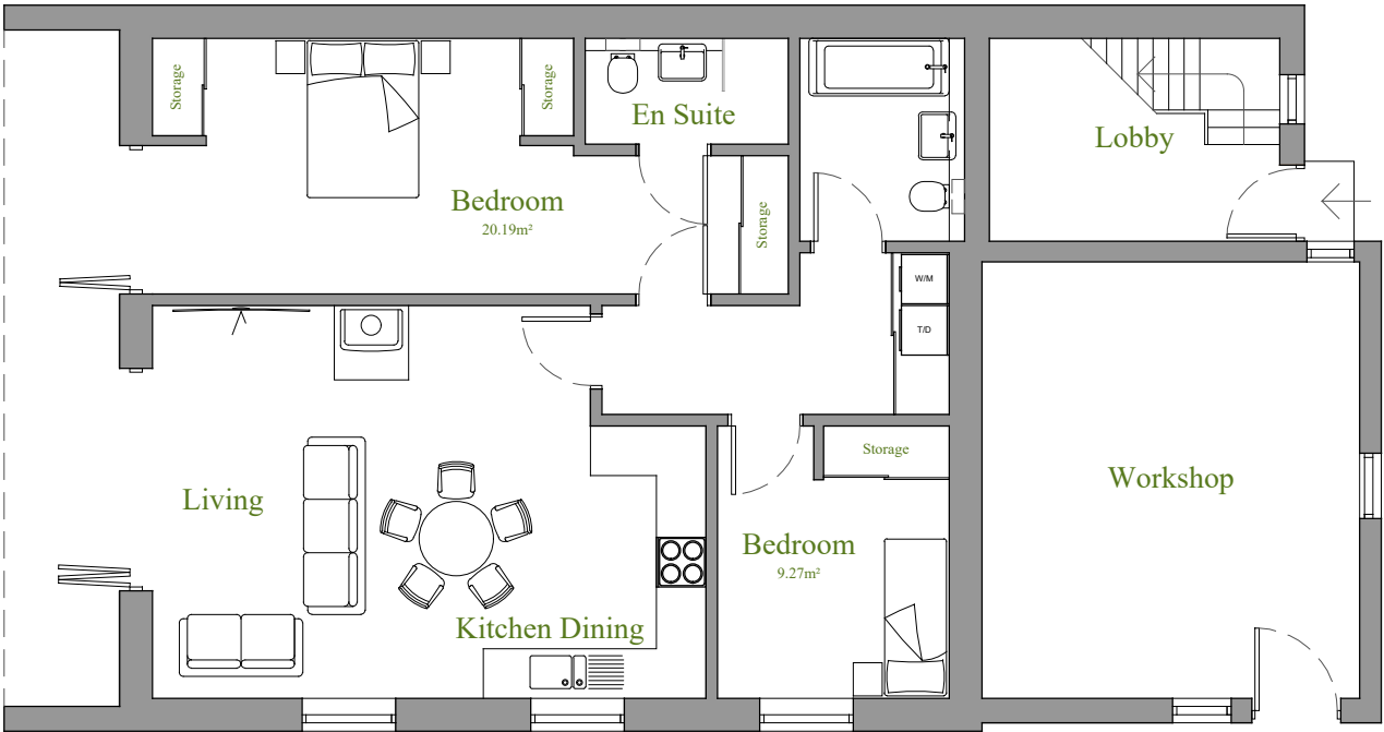
Ground Floor Plan 1:100 | APPROVED
