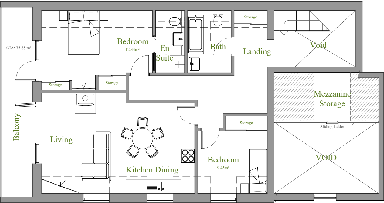
First Floor Plan 1:100 | PROPOSED
