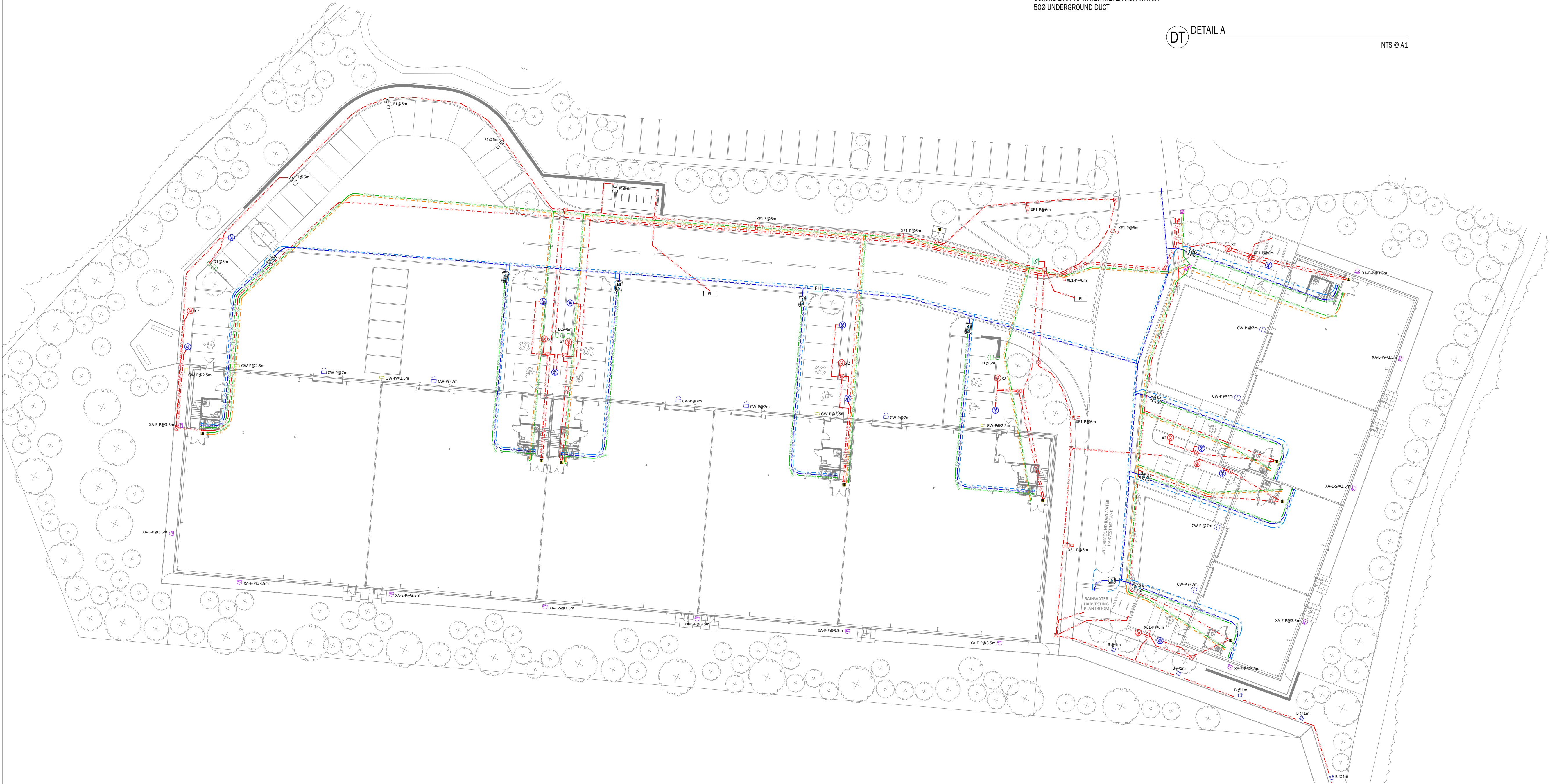
TYPICAL SERVICES UNDER PAVEMENT TO JVG V1 FIGURE 1 (N758A1)
