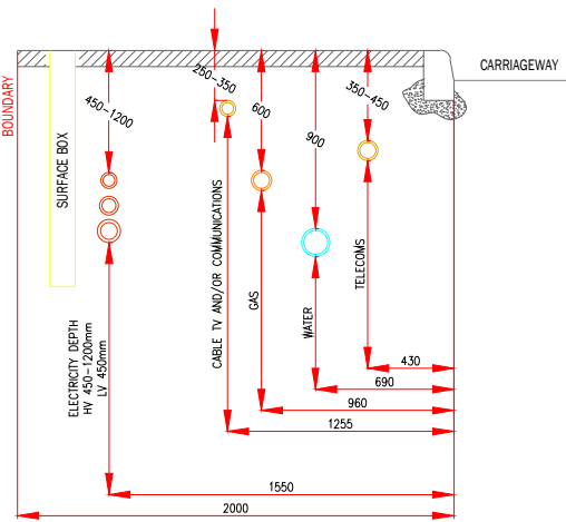
TYPICAL SERVICES UNDER PAVEMENT TO JVG V1 FIGURE 1 (N758A1)
