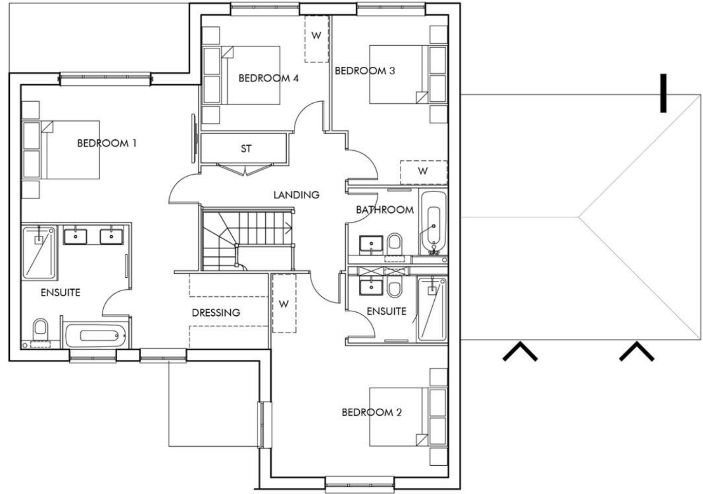
FIRST FLOOR
