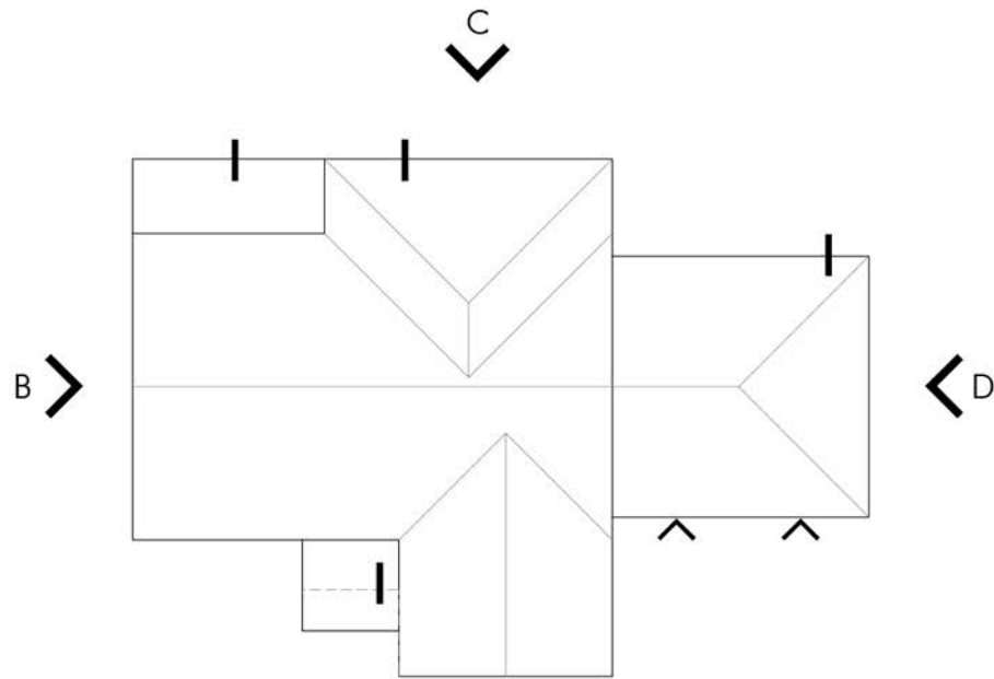
ROOF PLAN 1:200
