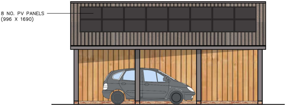
SIDE ELEVATION (SOUTH)
