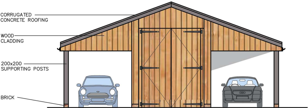
FRONT ELEVATION (WEST)
