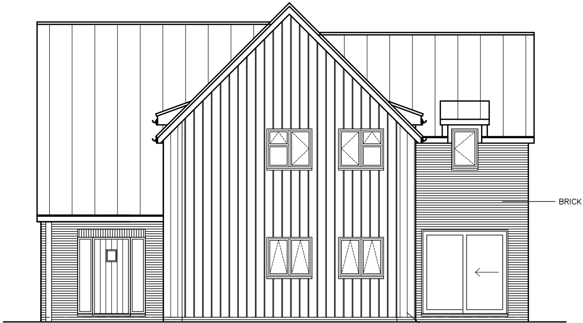
FRONT ELEVATION (SOUTH)
