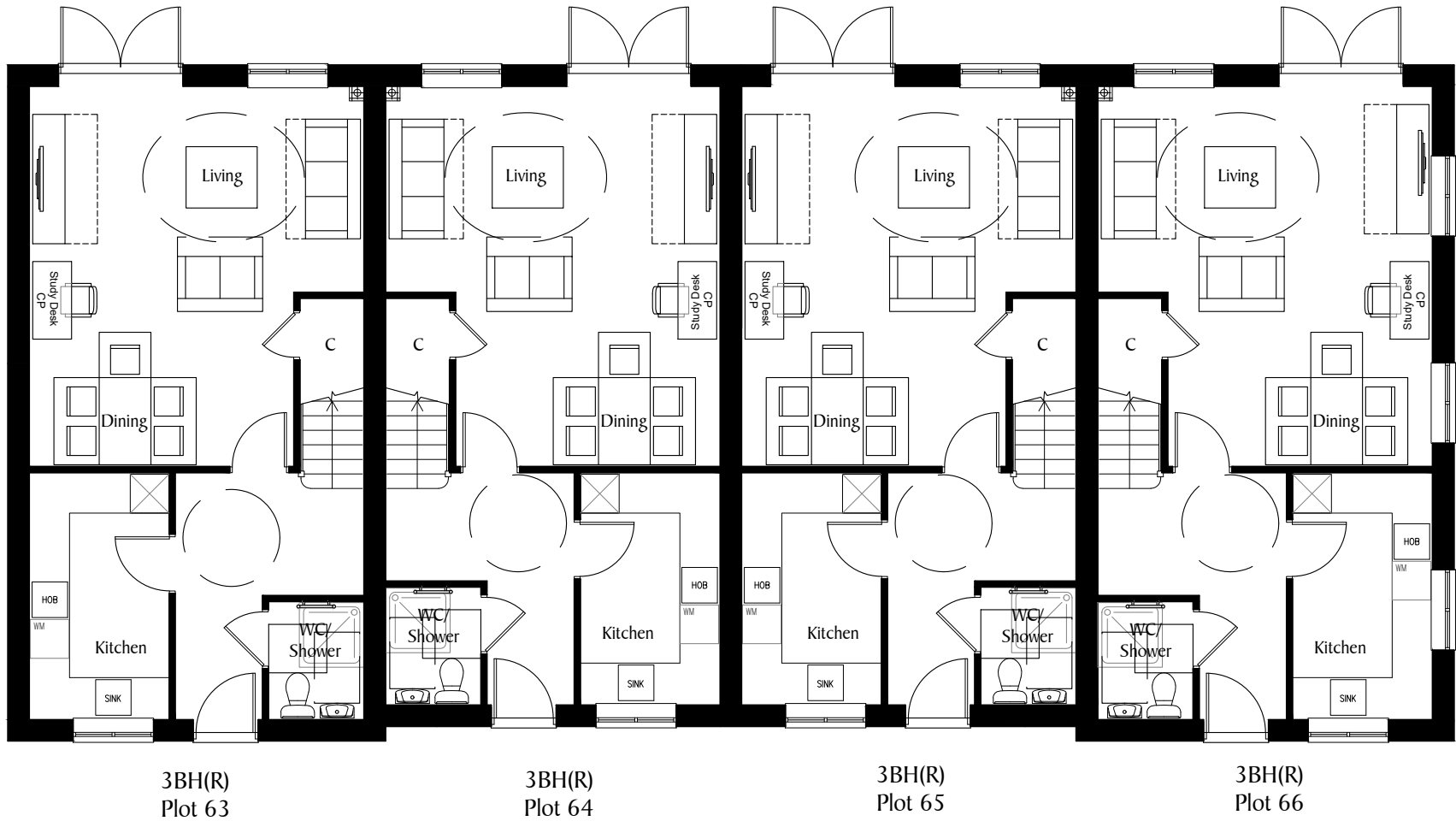
Ground Floor
