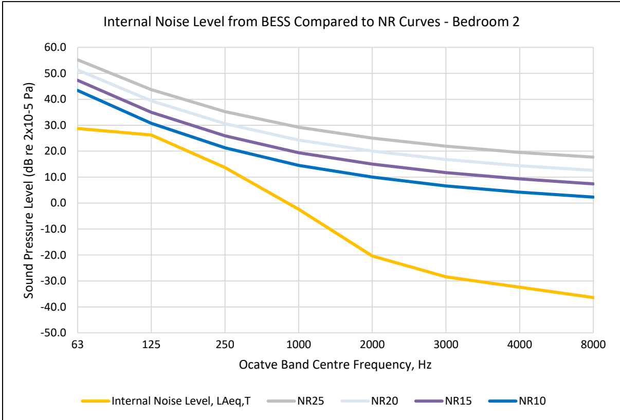
Figure 6-6: BESS Internal Noise Level Assessment – Bedroom 2
