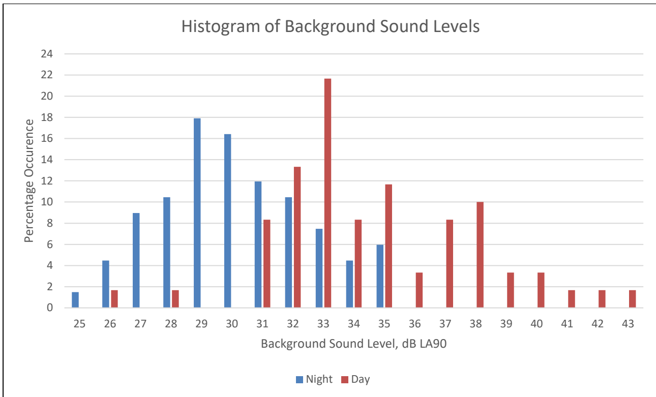
Figure 6-3: Histogram of Background Sound Levels
