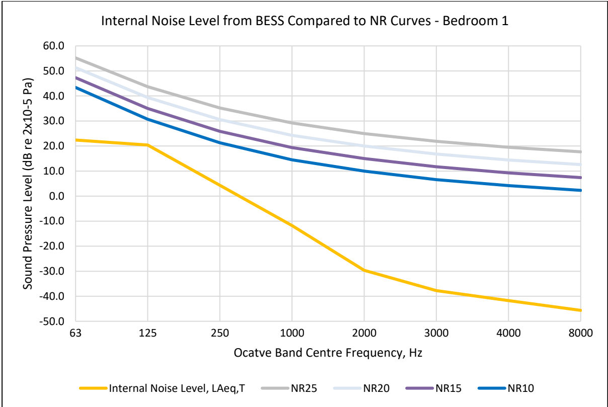
Figure 6-5: BESS Internal Noise Level Assessment – Bedroom 1
