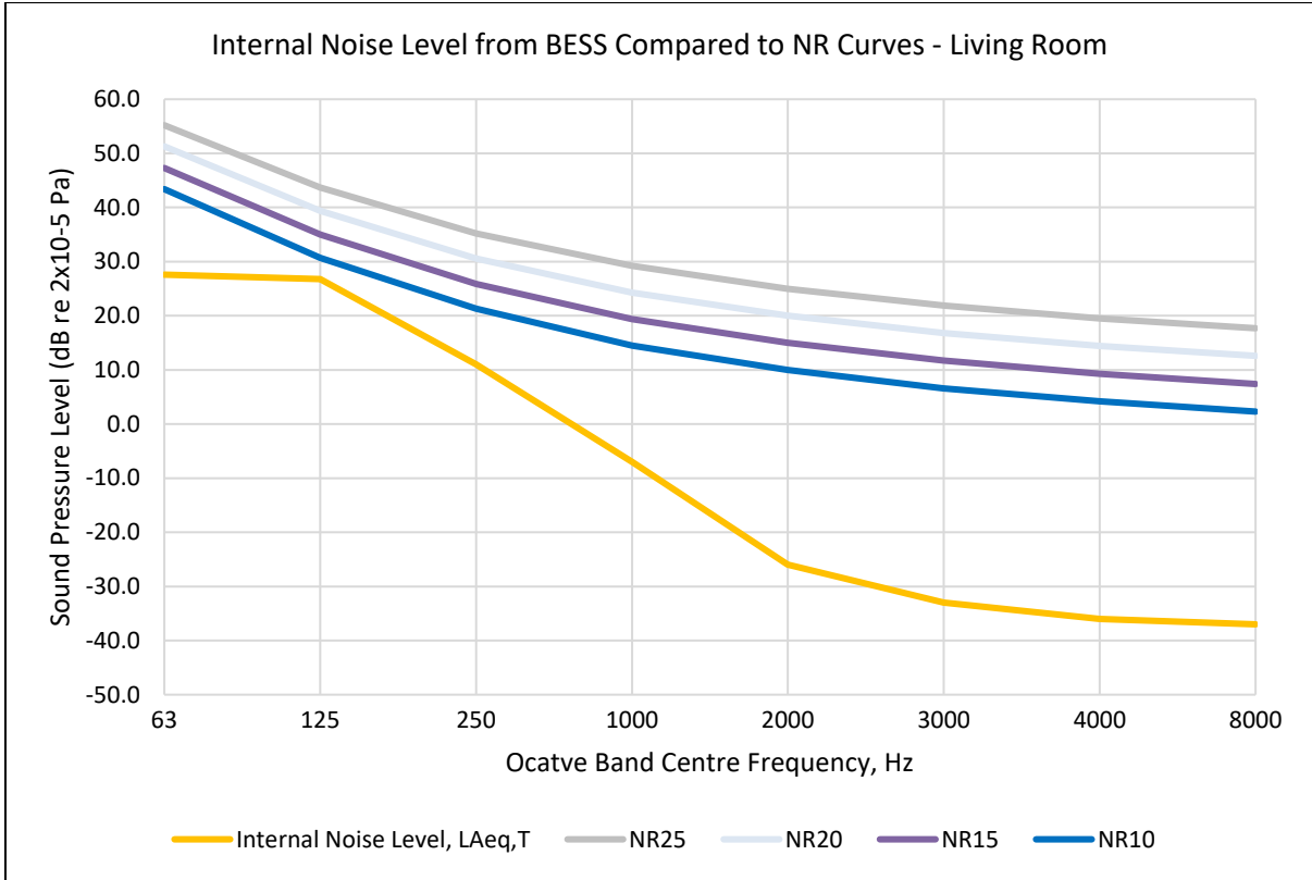
Figure 6-4: BESS Internal Noise Level Assessment – Living Room
