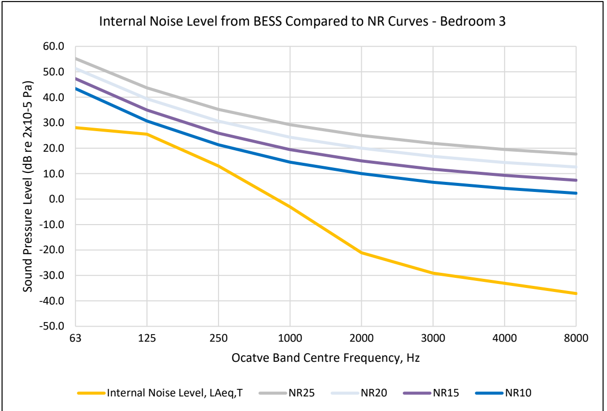
Figure 6-7: BESS Internal Noise Level Assessment – Bedroom 3
