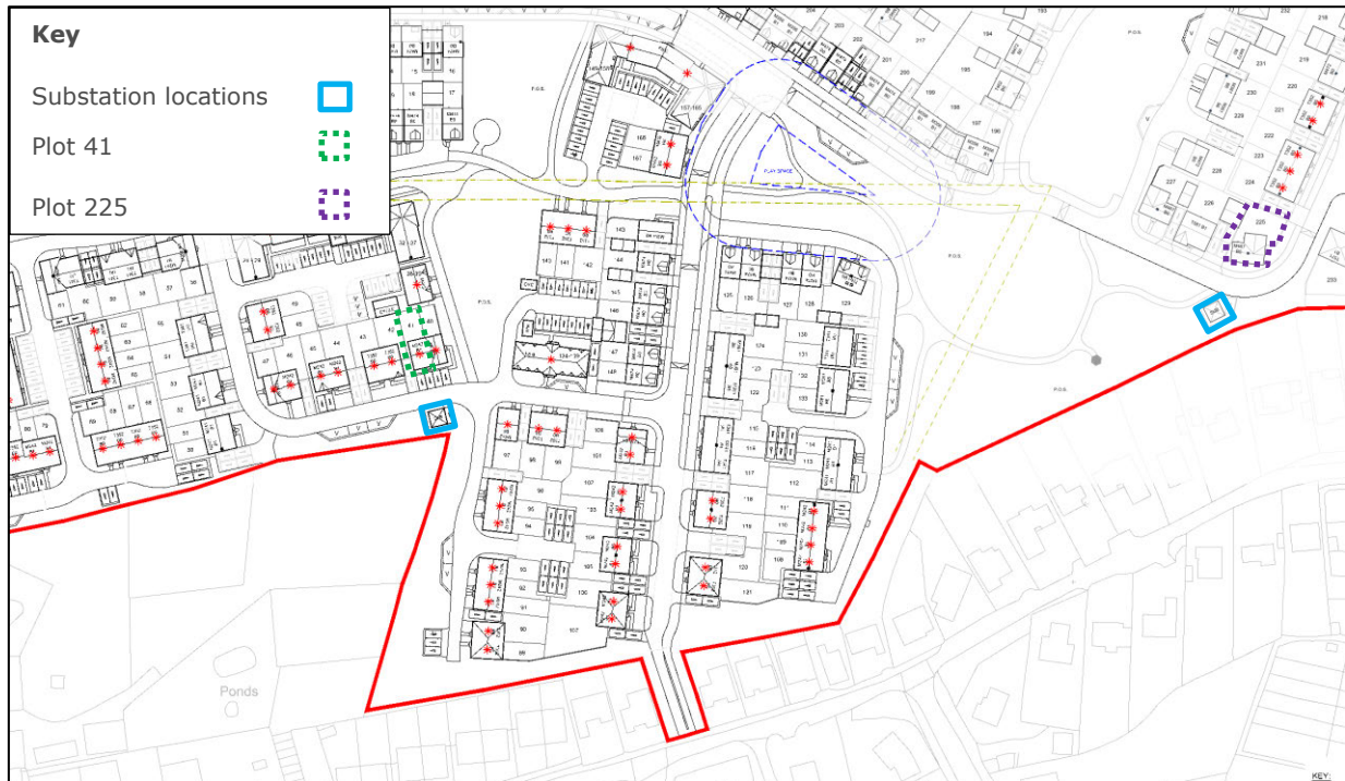
Figure 7-1: Substation Locations
