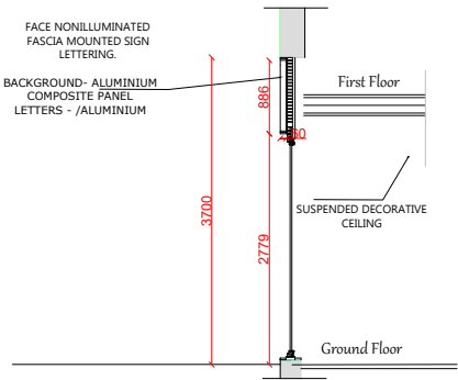
PROPOSED SIGN SECTION A-A
