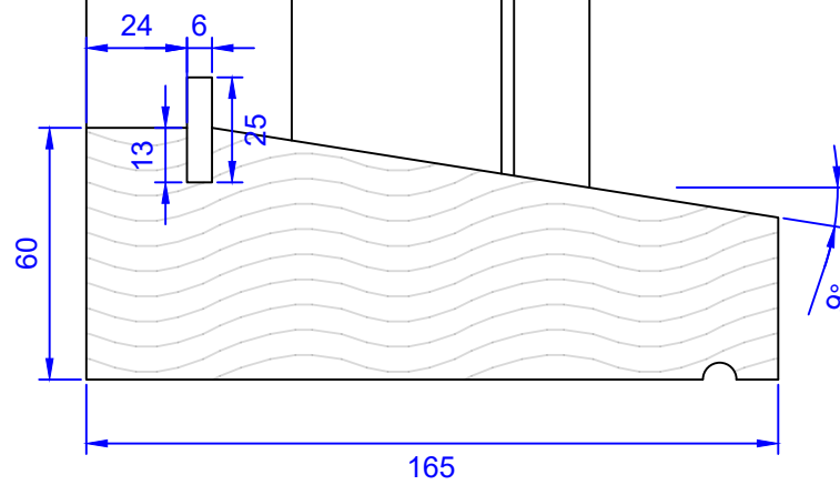
Cill Section
