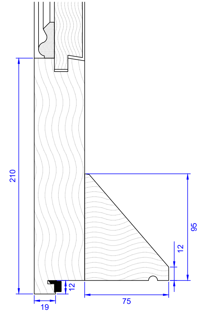
Bottom Rail Section
