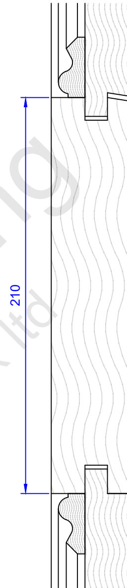
Middle Rail Section
