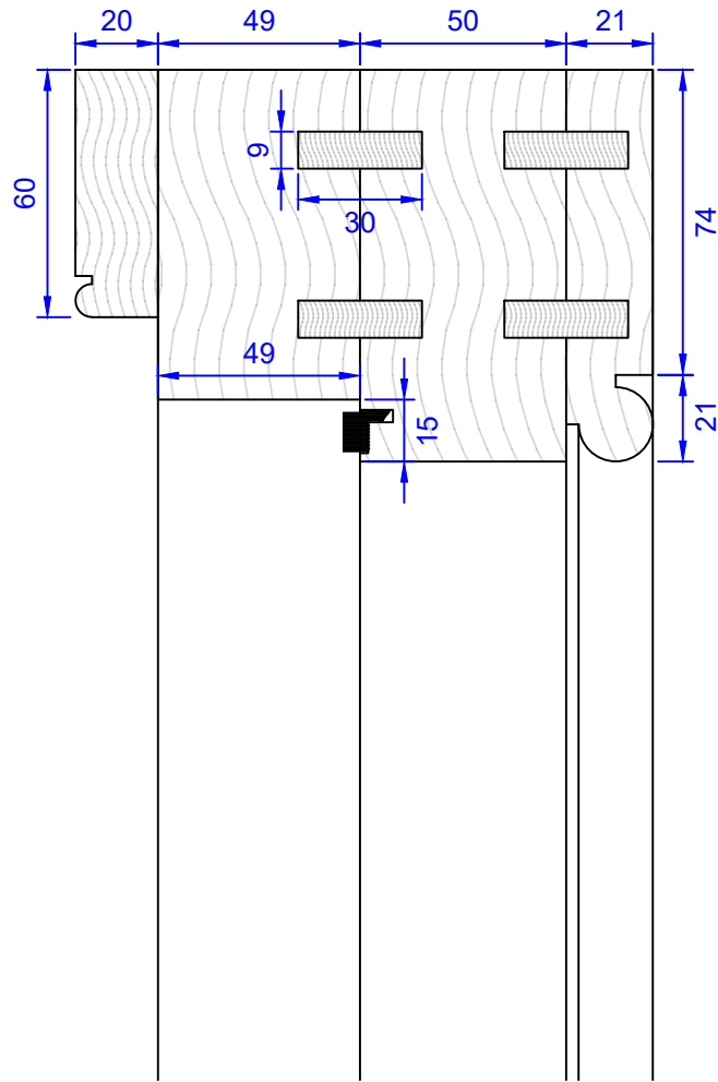
Head Section
