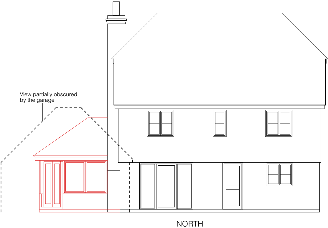
PROPOSED ELEVATIONS new works lined red
