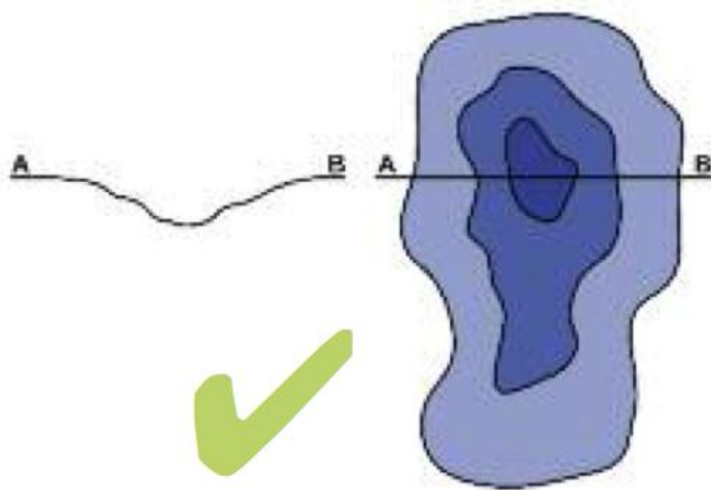
Figure 12. Design of SUDs showing varying depths at a gently sloping level (Freshwater Habitats 2013)
