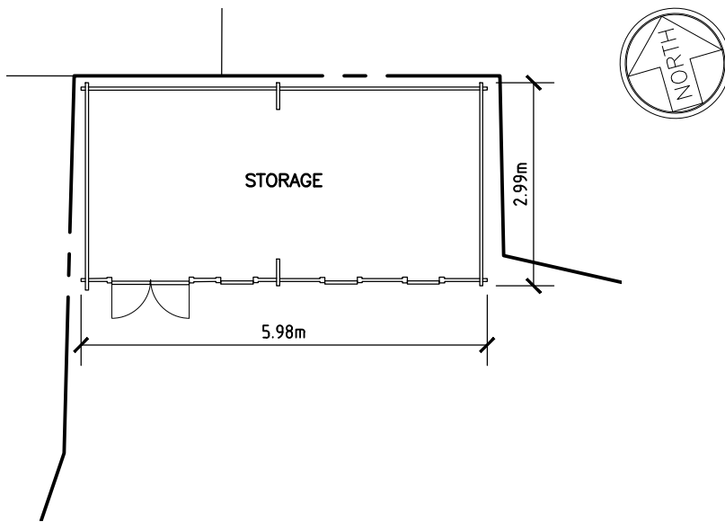
1. PROPOSED FLOOR 1:100
