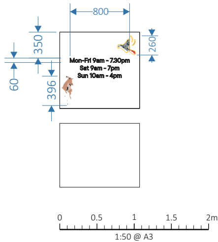
ITEM E EXISTING- 1:50 Scale Layered printed vinyl text & illustration, machine cut out and applied internally to glazed panels.
