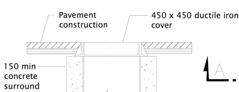
Alternative Cover Detail Medium/Heavy Duty
