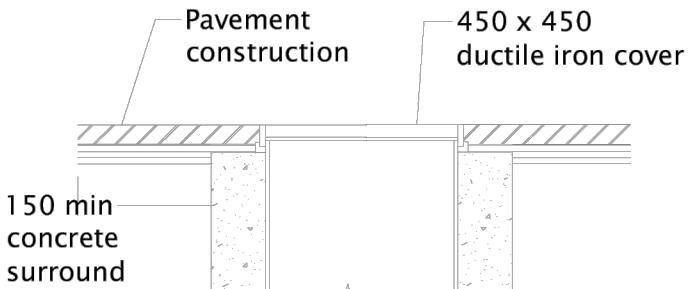
Alternative Cover Detail Light Duty
