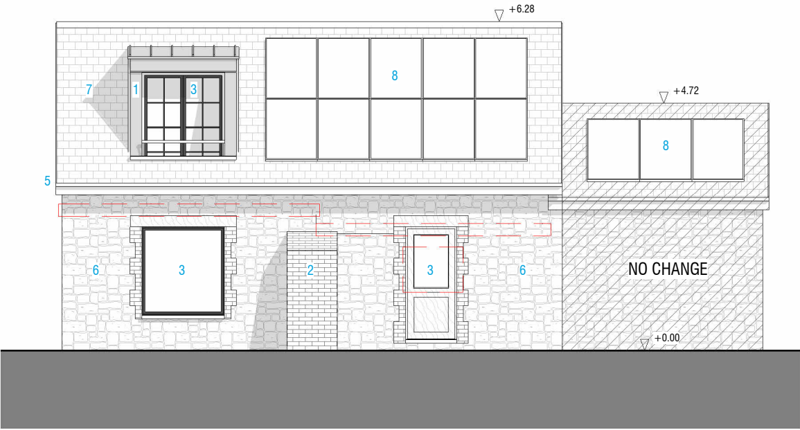
1 OUTBUILDING - PROPOSED FRONT 1 : 100
