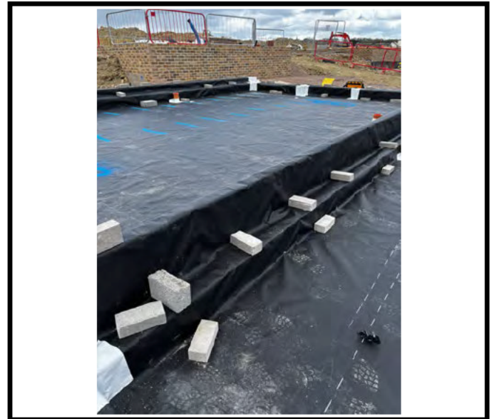
The JUTA GP1 Gas Barrier taken over the internal cavities to ensure continuity throughout.
