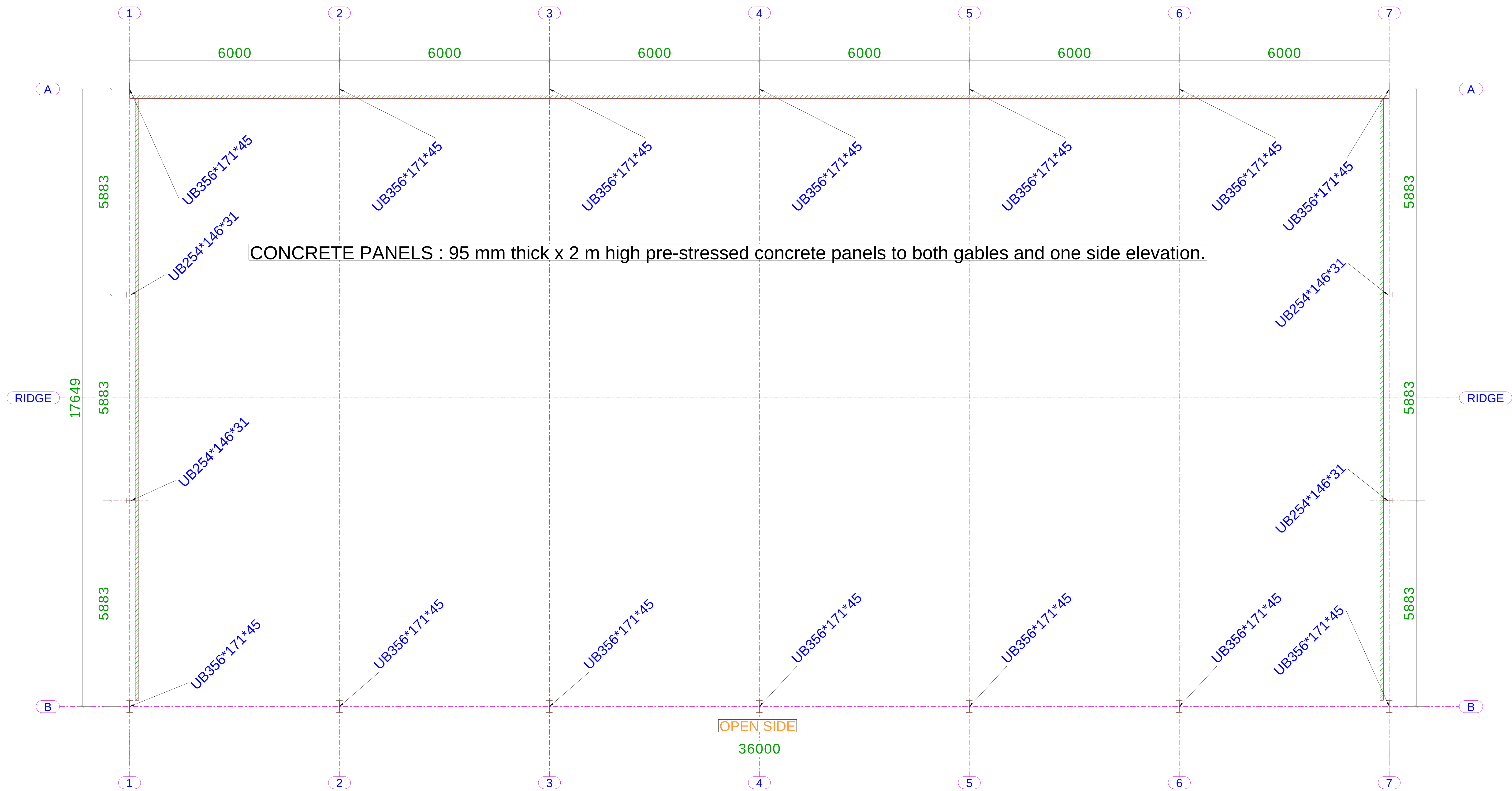
COLUMN LAYOUT SCALE 1 : 50 @ A0
