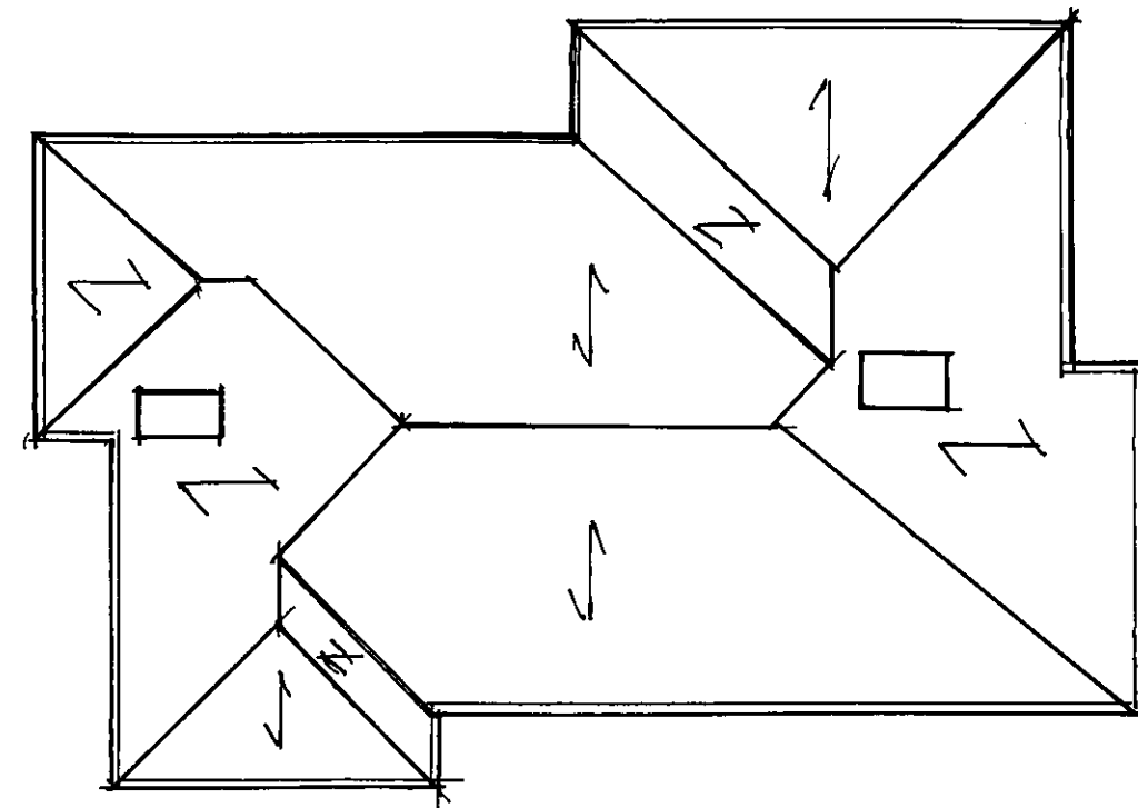
ROOF PLAN
