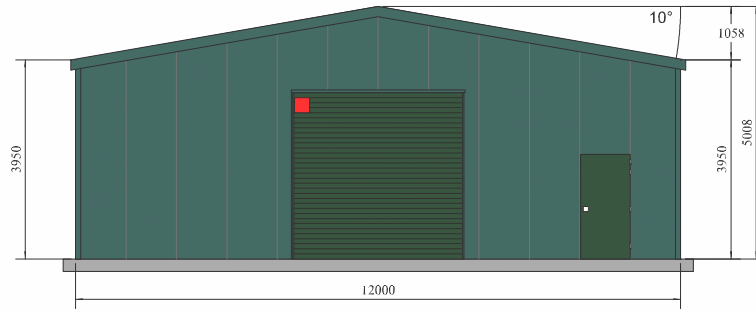
FRONT ELEVATION (EXTERNAL)
