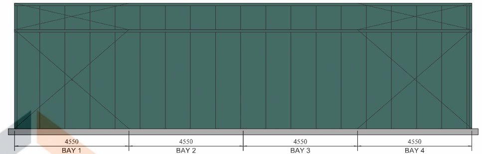
LEFT ELEVATION VIEWED FROM INSIDE
