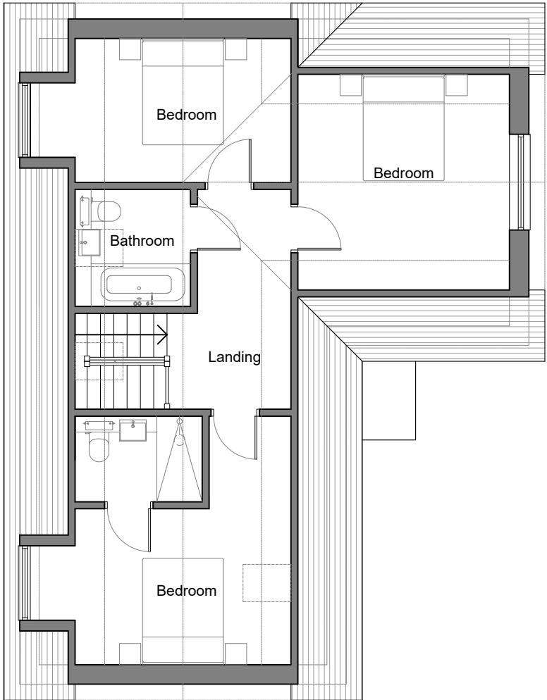
First Floor Plan 1:100 @ A1
