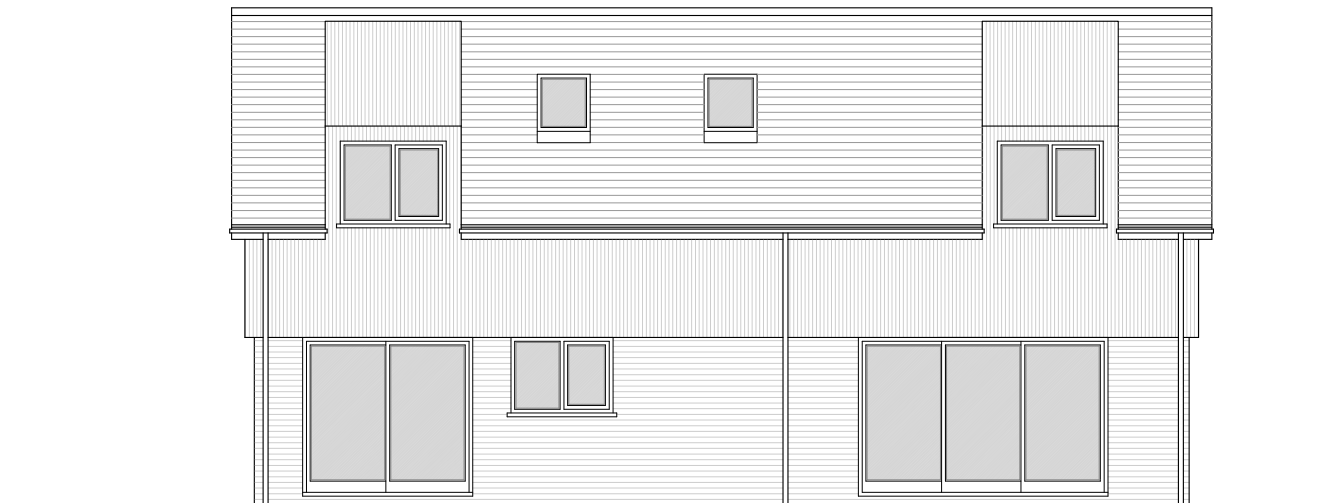
South Elevation 1:100 @ A1
