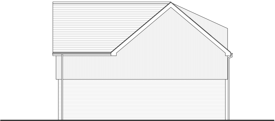
West Elevation 1:100 @ A1
