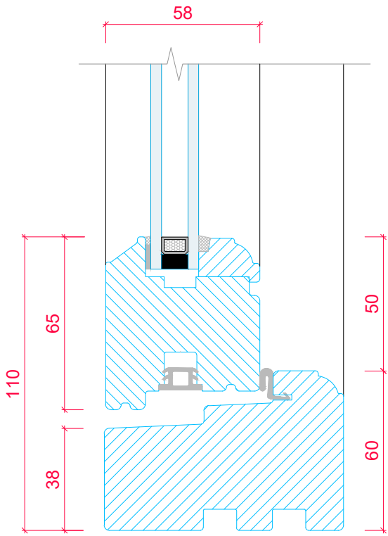
CASEMENT CROSS SECTION 'A-A' (SCALE 1:2)
