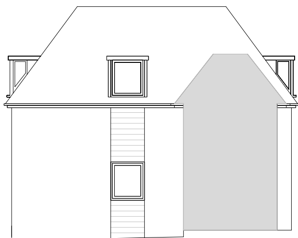
Existing East Elevation/Section
