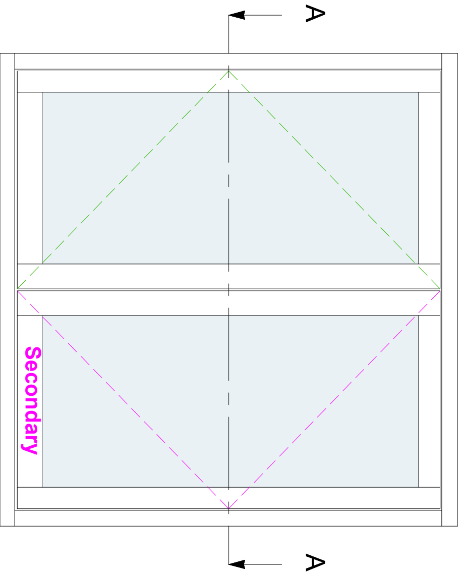
TYPICAL CASEMENT LAYOUT (SCALE 1:10)
