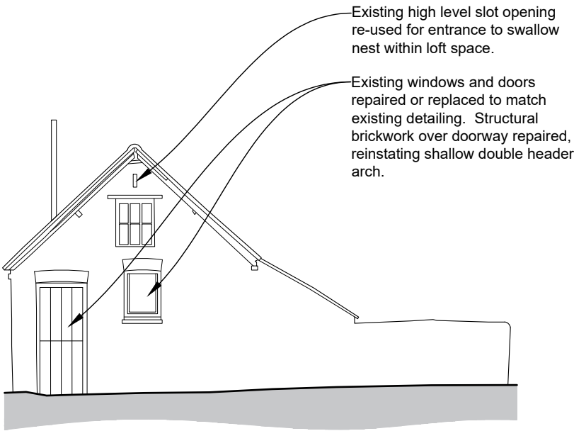
1 North Elevation Proposed 1:100
