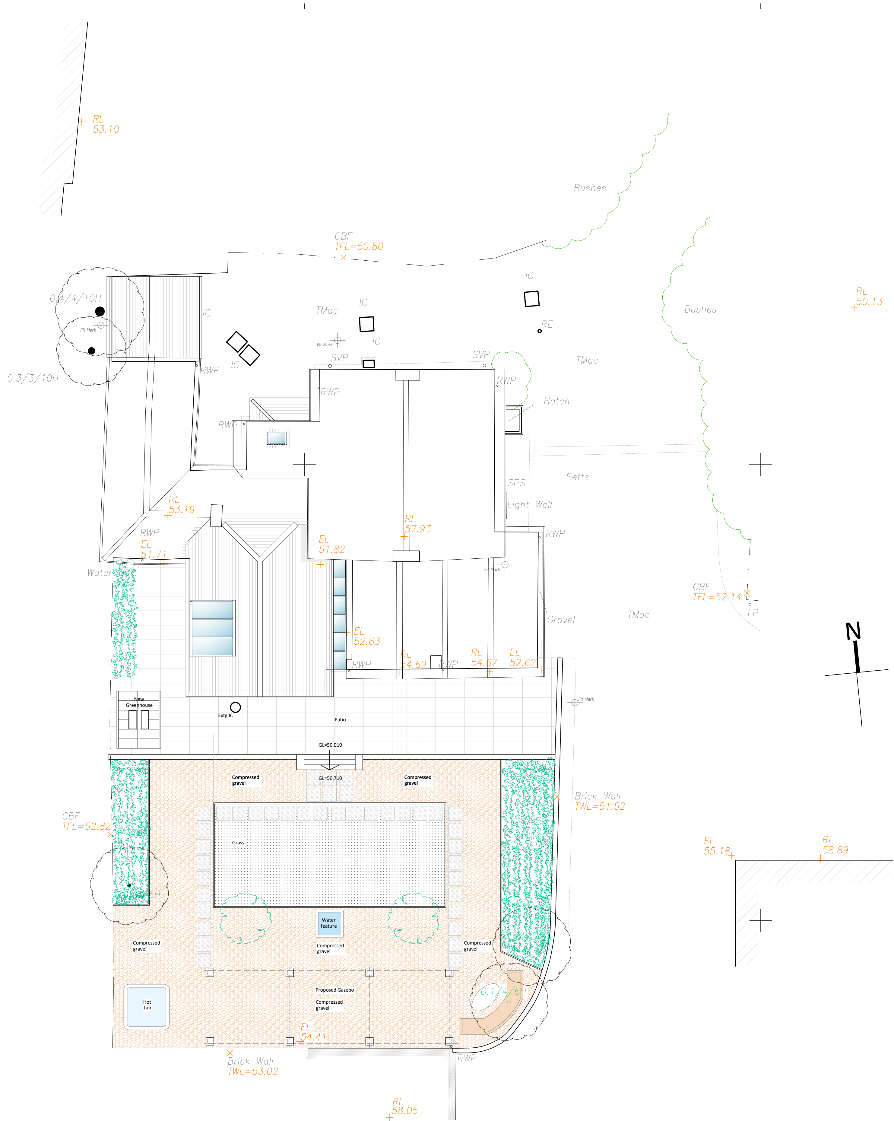
PROPOSED SITE LAYOUT PLAN
