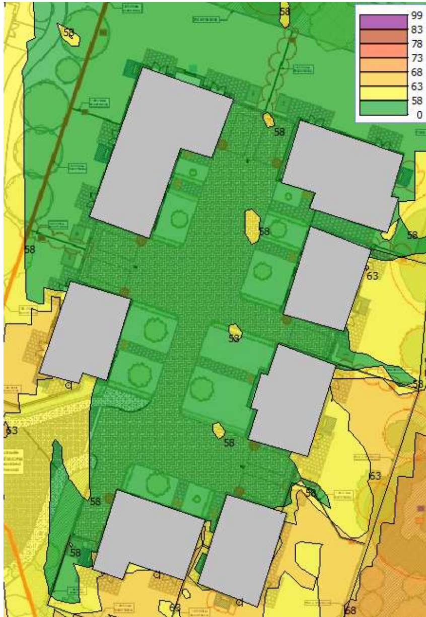
Figure 5.4 - Night Time LAmax, 2300 – 0700
