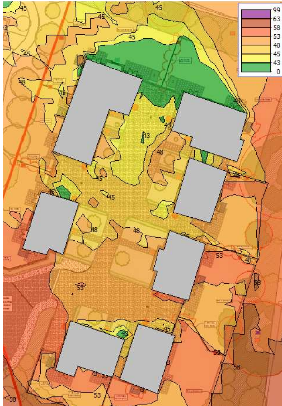
Figure 5.2 - Day Time LAeq, 07.00 – 23.00
