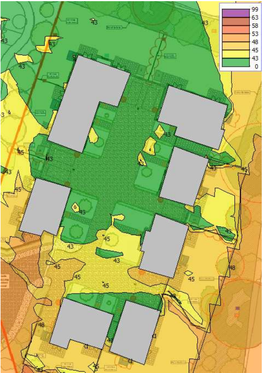
Figure 5.3 - Night Time LAeq, 23.00 – 07.00
