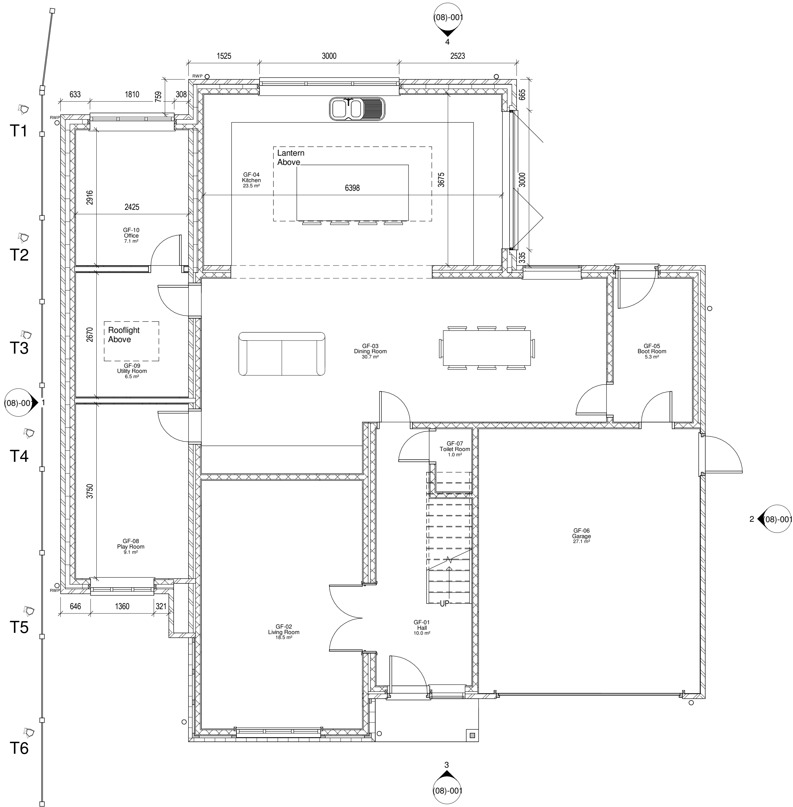
1 Ground Floor - Proposed Plan 1 : 50
