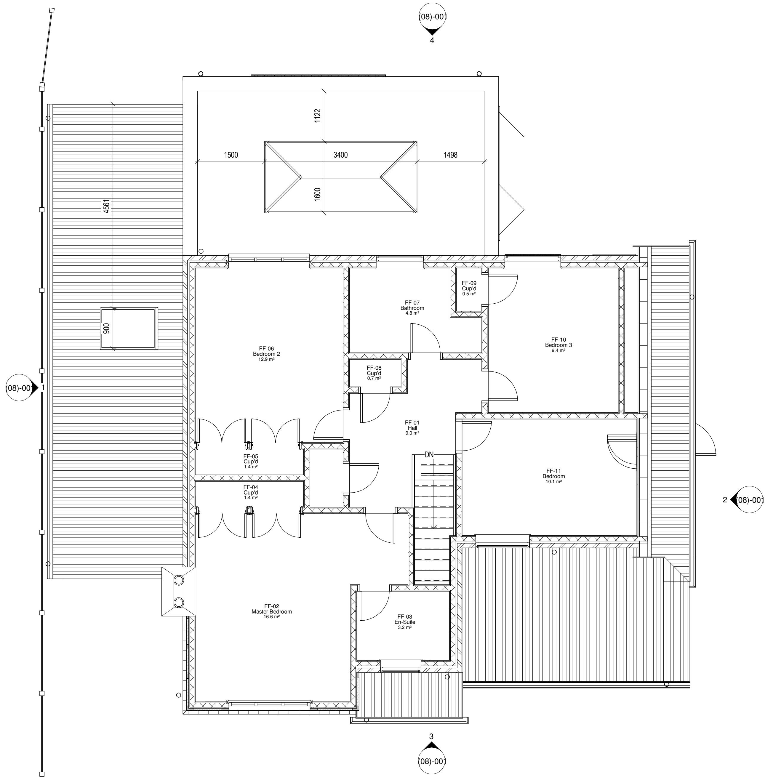
2 First Floor - Proposed Plan 1 : 50
