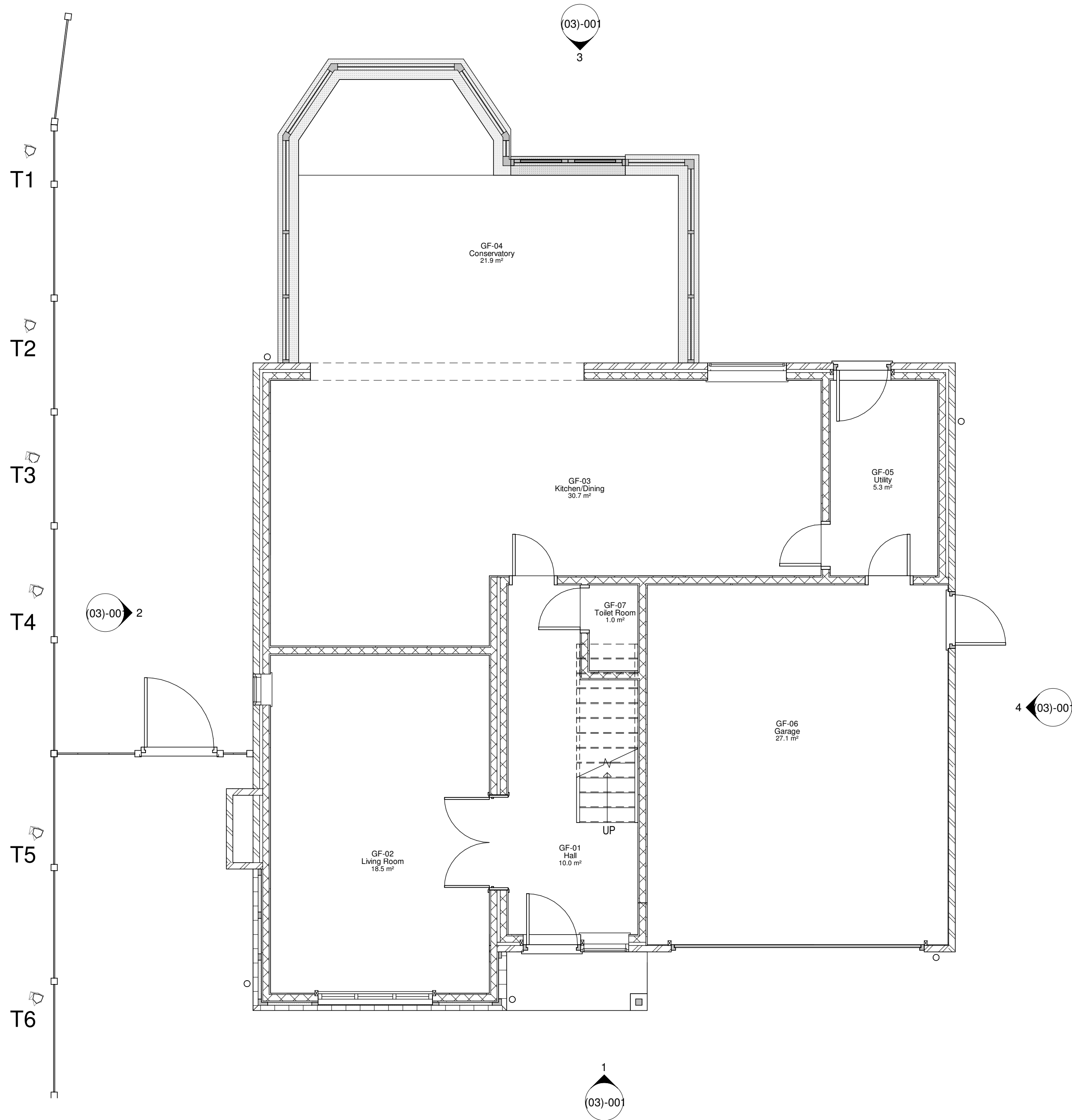
1 Ground Floor - Existing Plan 1 : 50
