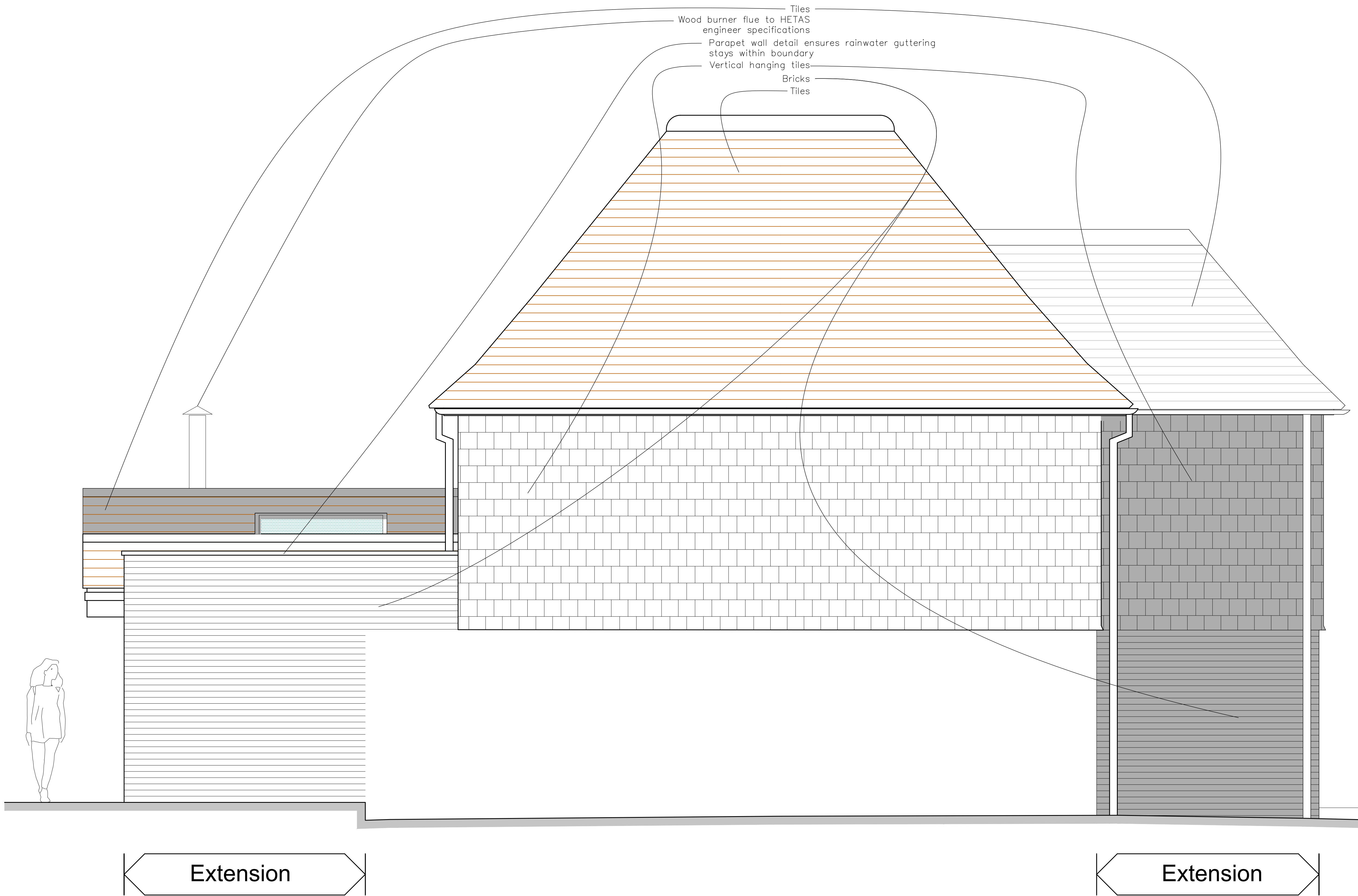
PROPOSED SIDE ELEVATION (east) Scale 1:25
