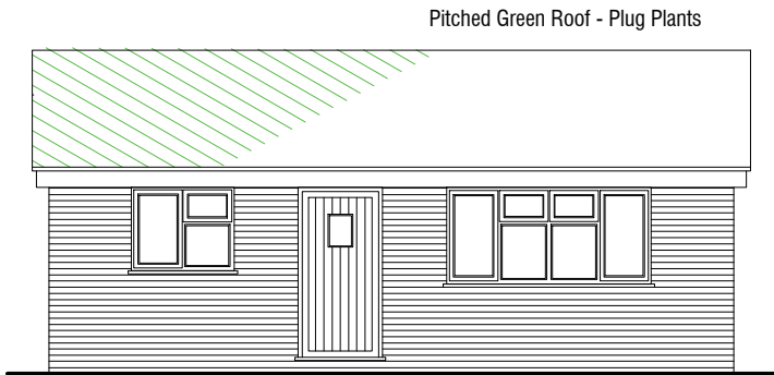
PROPOSED FRONT ELEVATION (DAY ROOM) Scale 1:100
