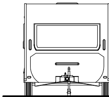
PROPOSED FRONT ELEVATION (TOURING CARAVAN) Scale 1:100
