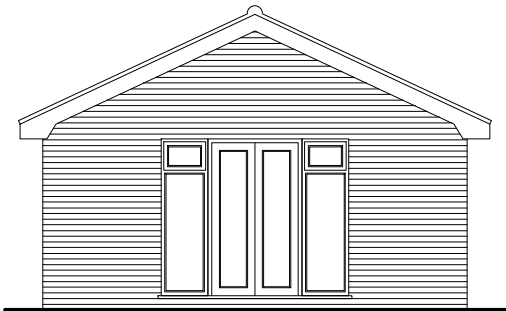
PROPOSED SIDE ELEVATION (DAY ROOM) Scale 1:100
