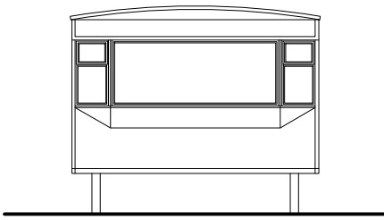
PROPOSED FRONT ELEVATION (STATIC CARAVAN) Scale 1:100
