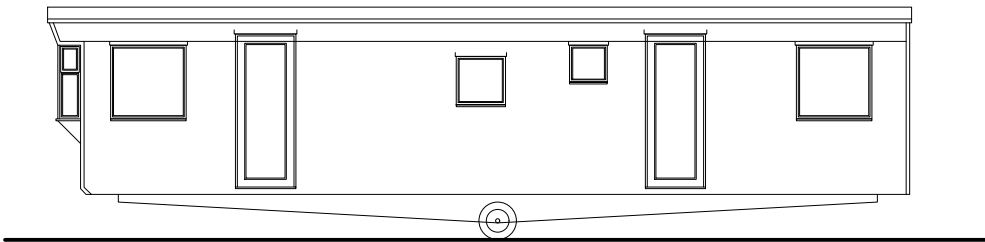
PROPOSED SIDE ELEVATION (STATIC CARAVAN) Scale 1:100
