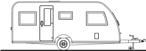
PROPOSED SIDE ELEVATION (TOURING CARAVAN) Scale 1:100
