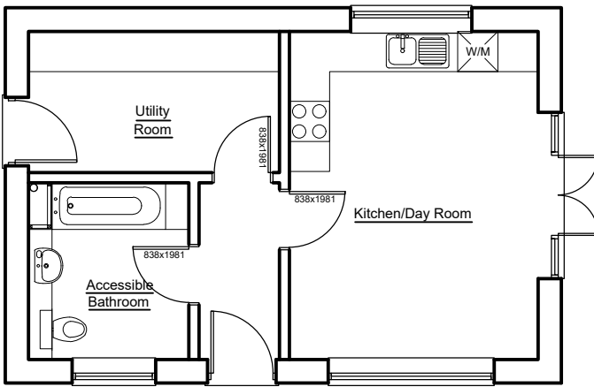
PROPOSED FLOOR PLAN (DAY ROOM) Scale 1:100
