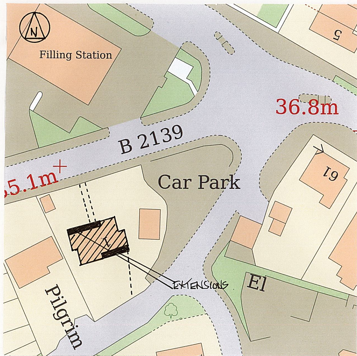
BLOCK PLAN
