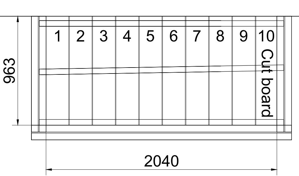
Balcony 17 - Second Floor
