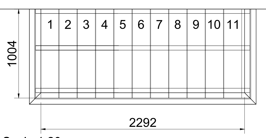
Balcony 19 - Second Floor
