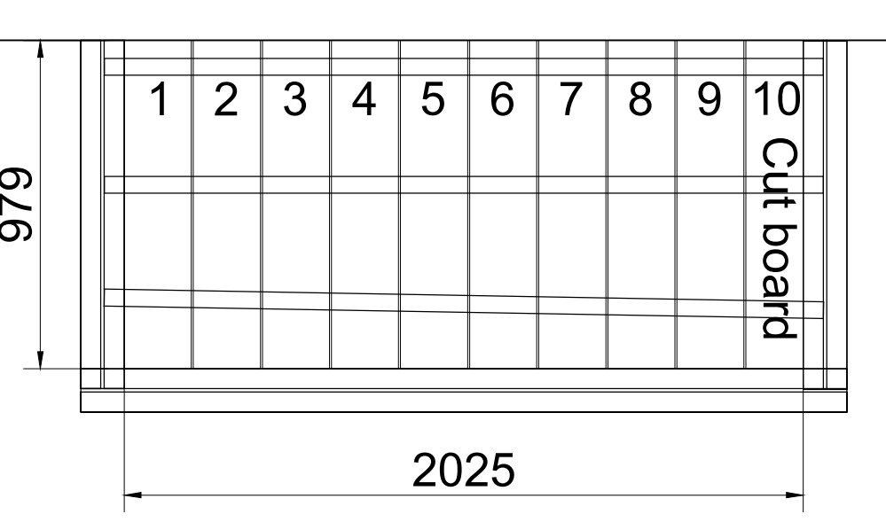
Balcony 18 - Second Floor
