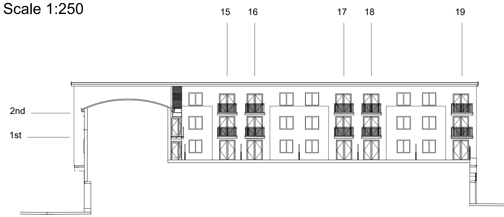
Balcony 17 - First Floor
