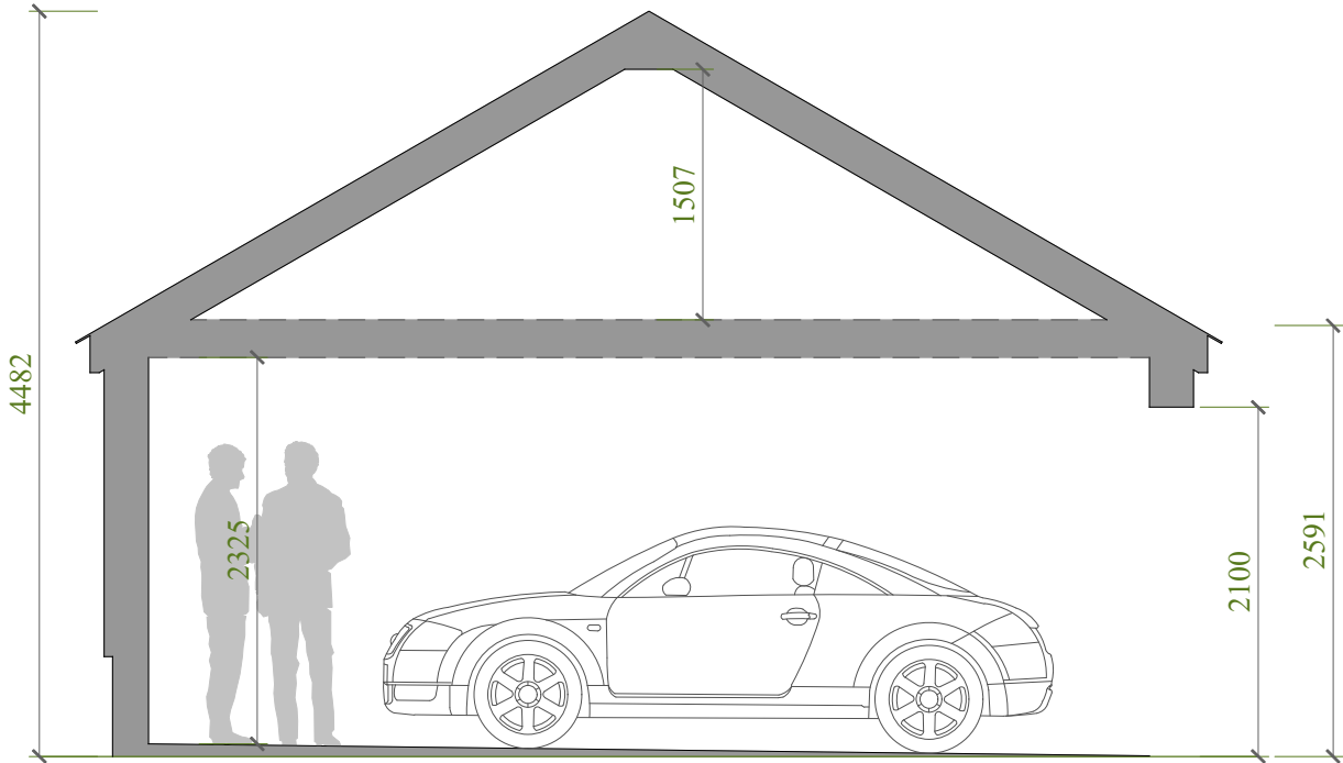
Garage Section EE
