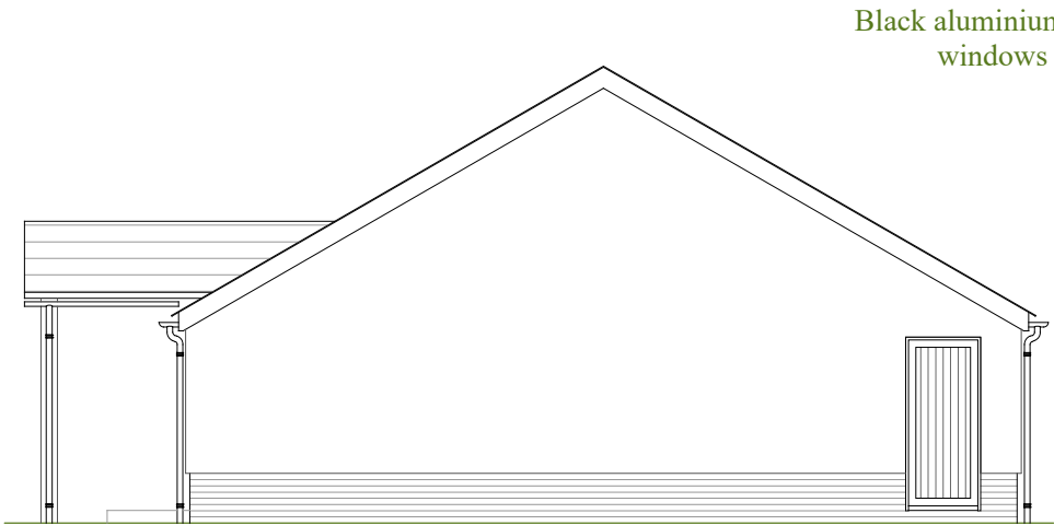
South 1:100 PROPOSED
