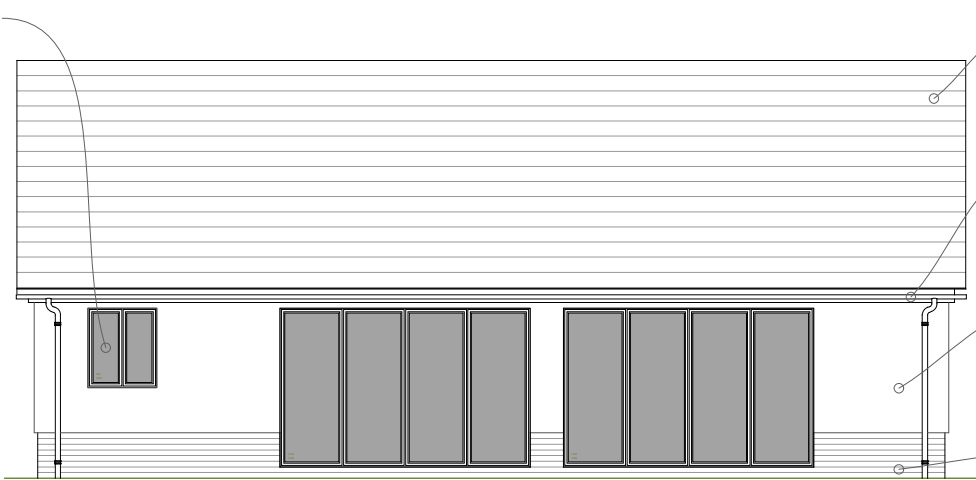
East 1:100 PROPOSED
