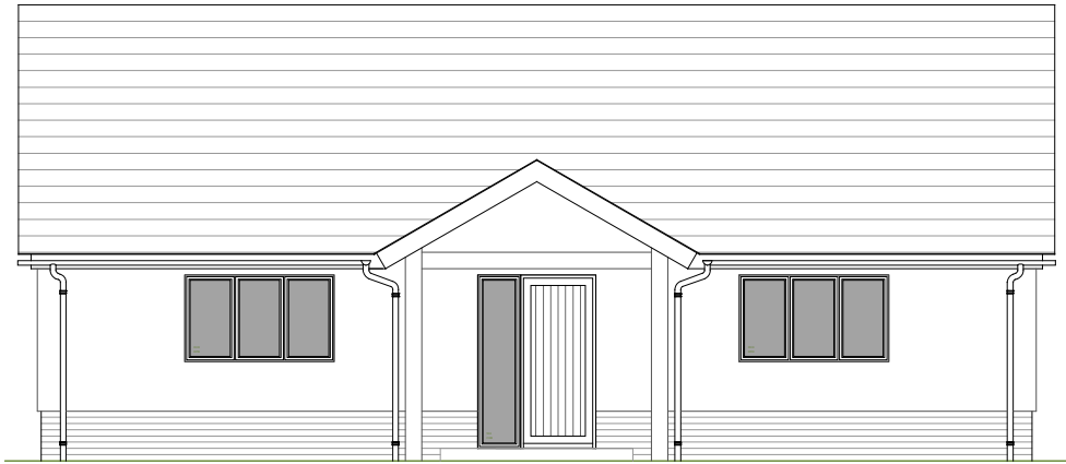
West 1:100 PROPOSED
