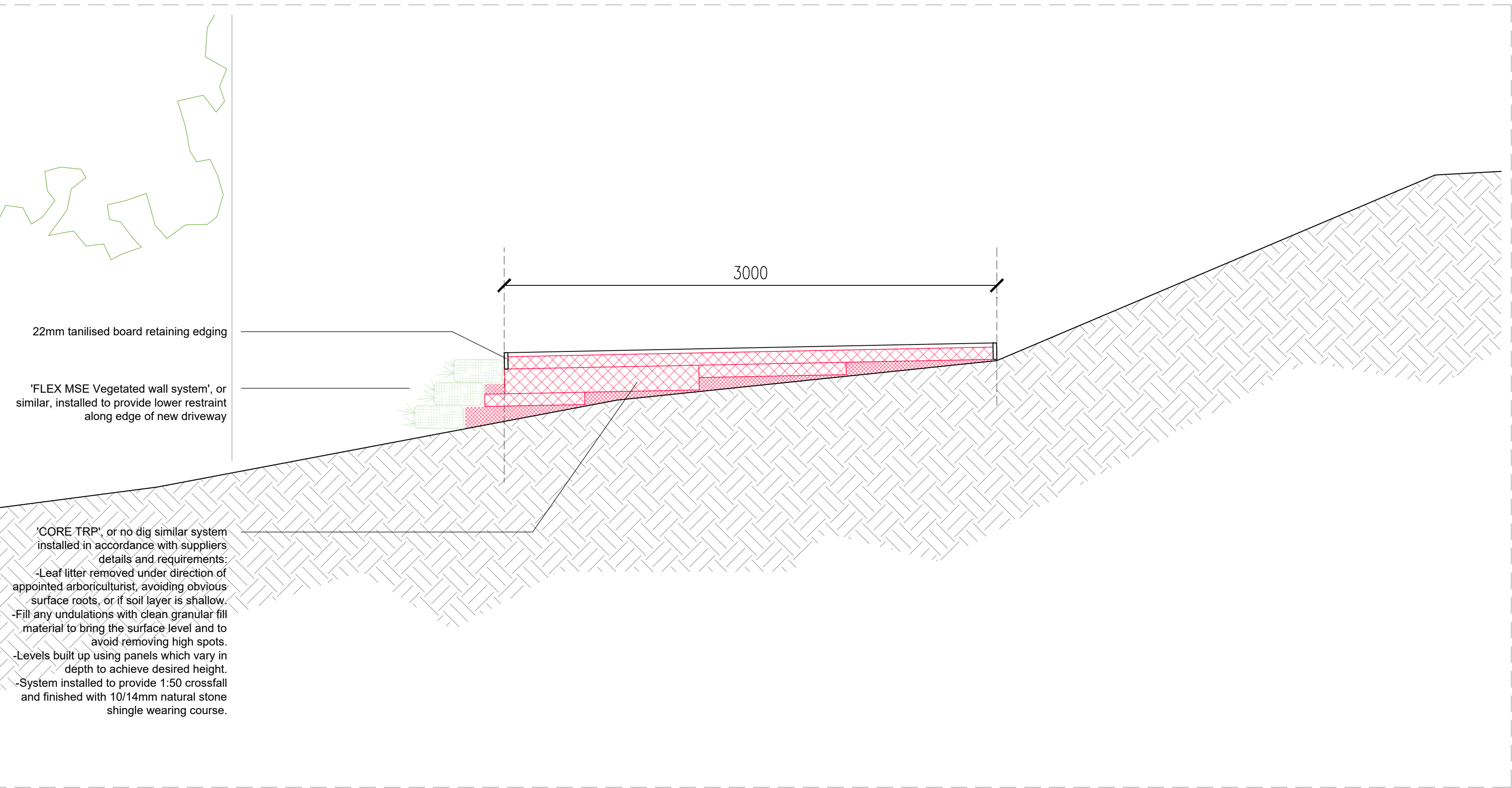
SECTION THROUGH DRIVEWAY
