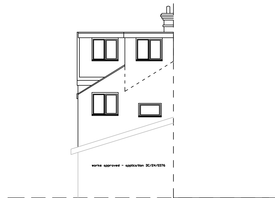
proposed eastern elevatioin
