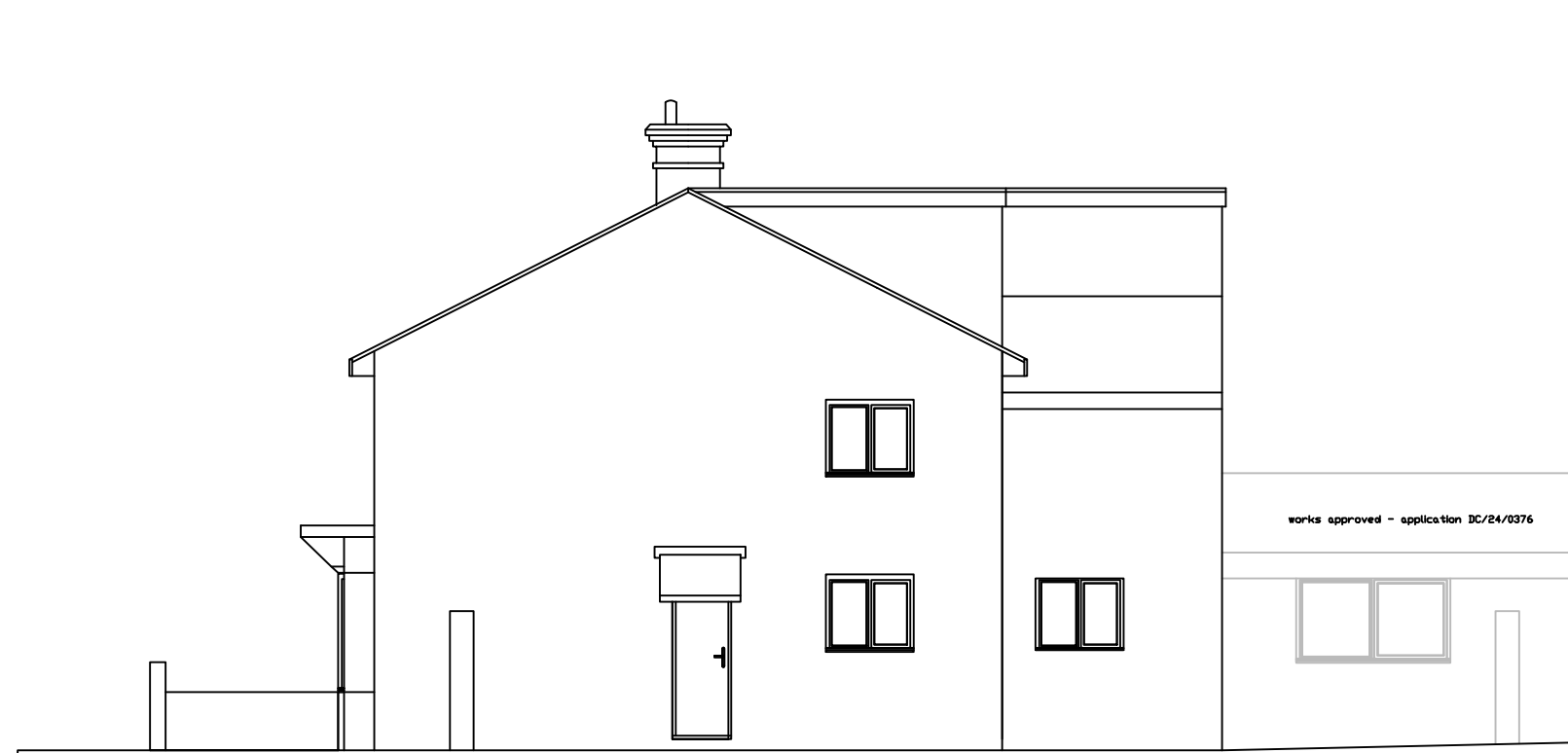
proposed southern elevation
