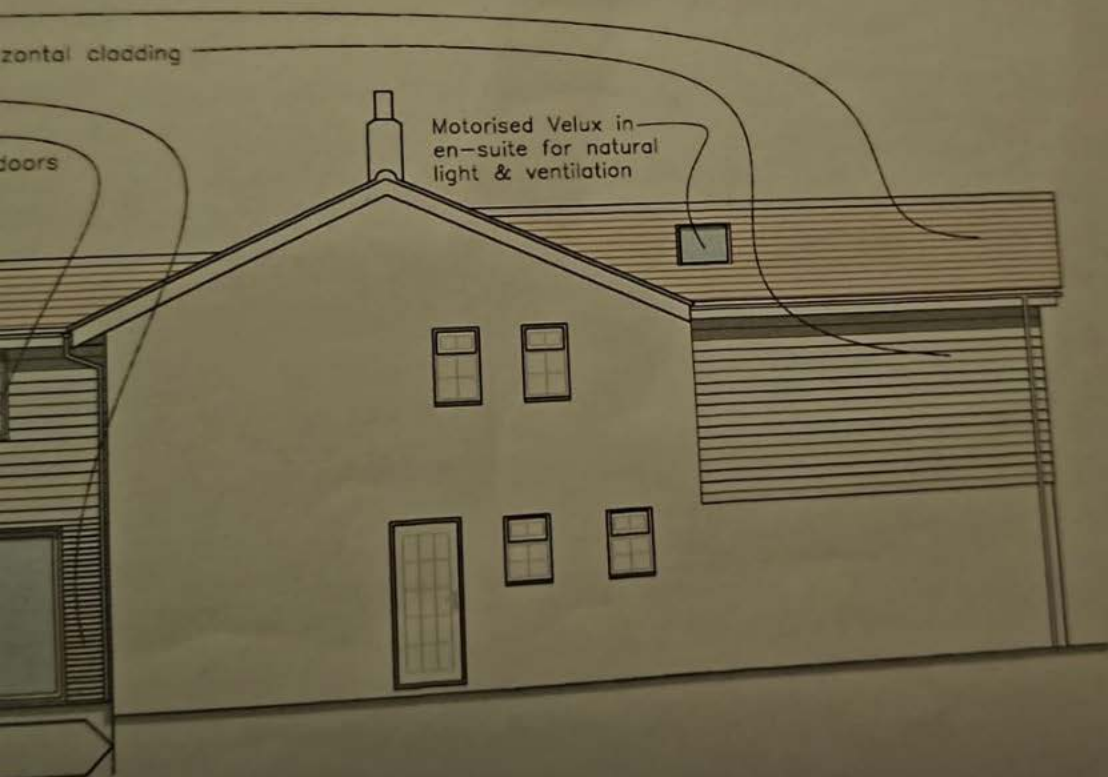
PROPOSED EAST ELEVATION (east) scale 1:20
