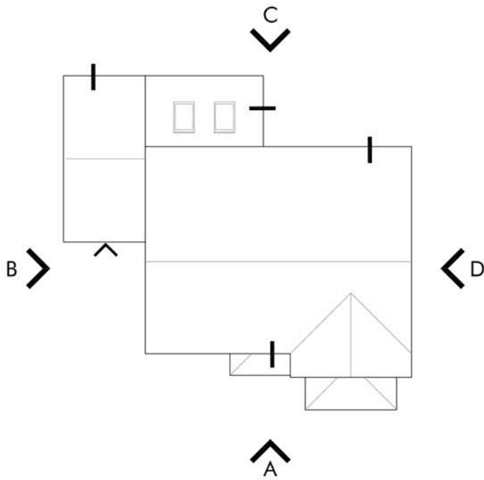
ROOF PLAN 1:200
