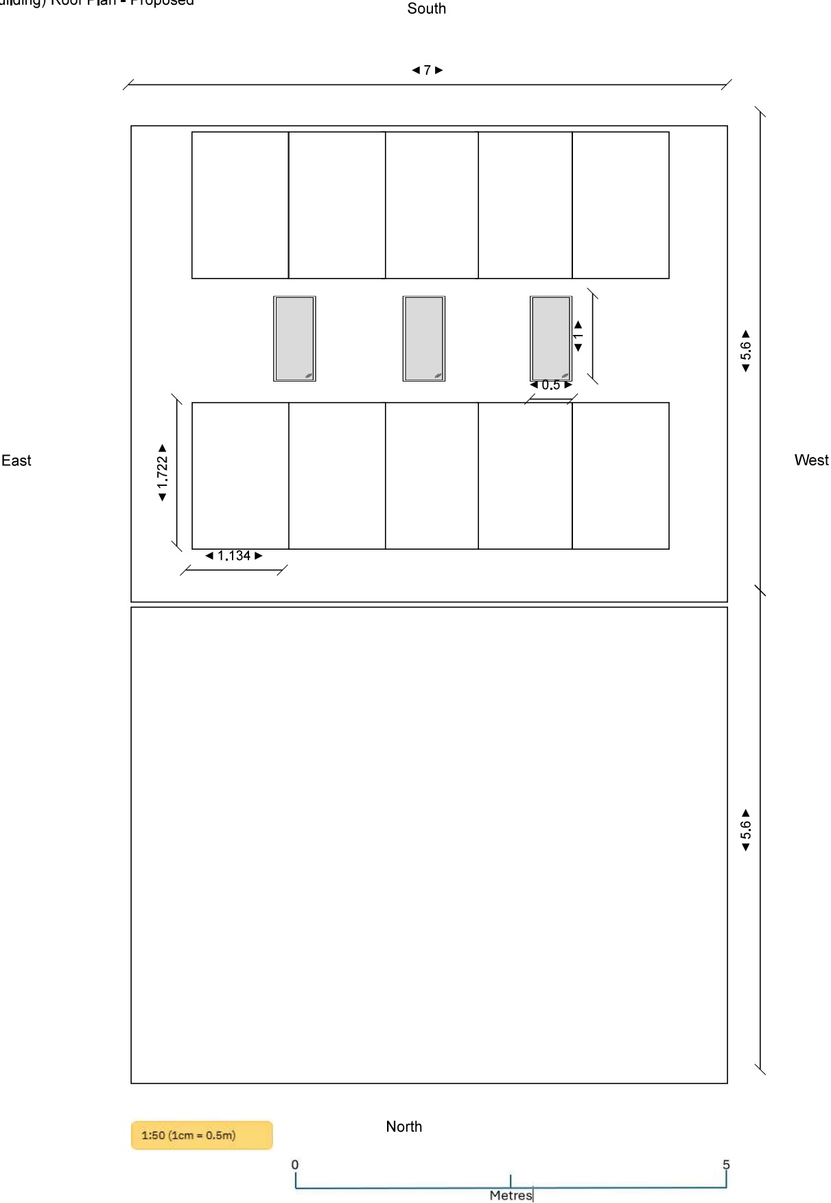
Barn (outbuilding) Roof Plan - Proposed
