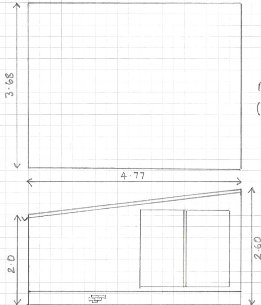
WEST ELEVATION
