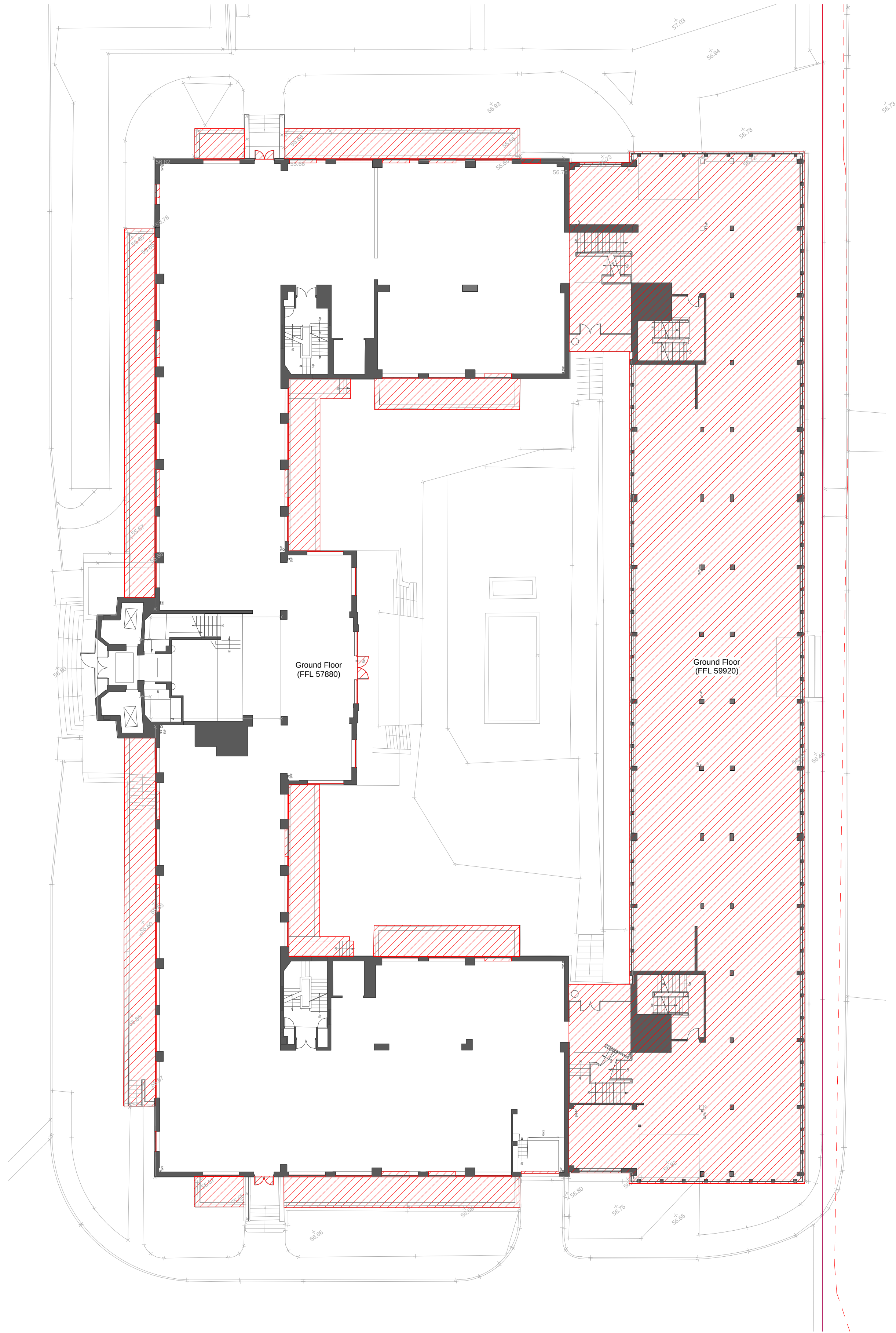
1 Existing Ground Floor Demolition Plan 1 : 200
