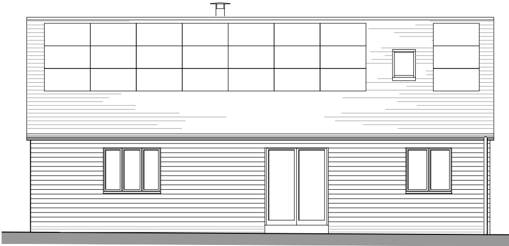
PROPOSED SOUTH ELEVATION 1:100
