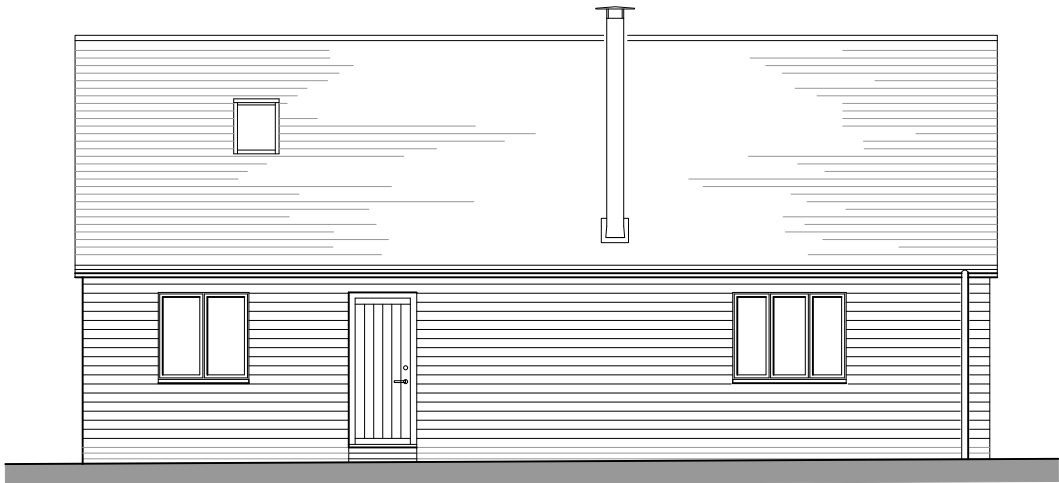
PROPOSED NORTH ELEVATION 1:100
