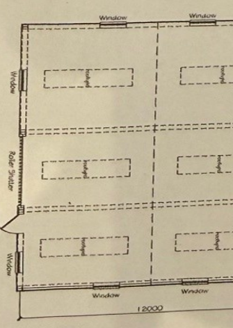
Ground Plan
