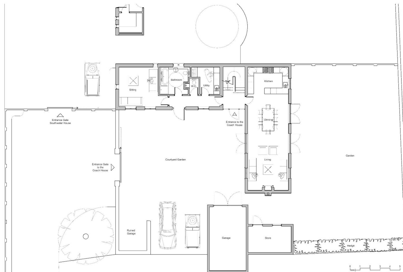
Ground floor plan of the proposed conversion and extension to the stable block
