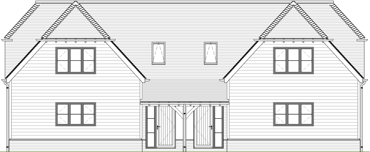
East 1:100 | PROPOSED
