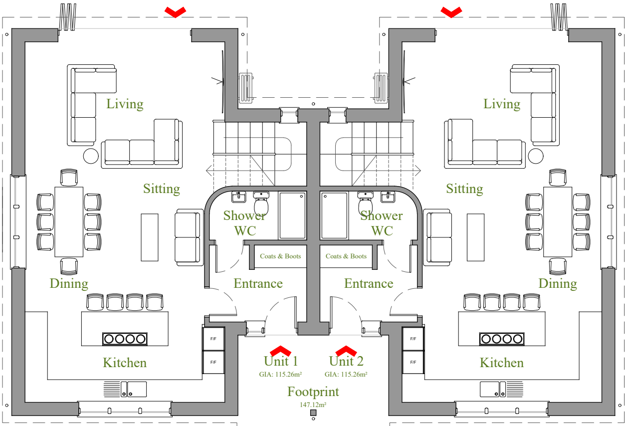
Ground Floor Plan 1:100 | PROPOSED
